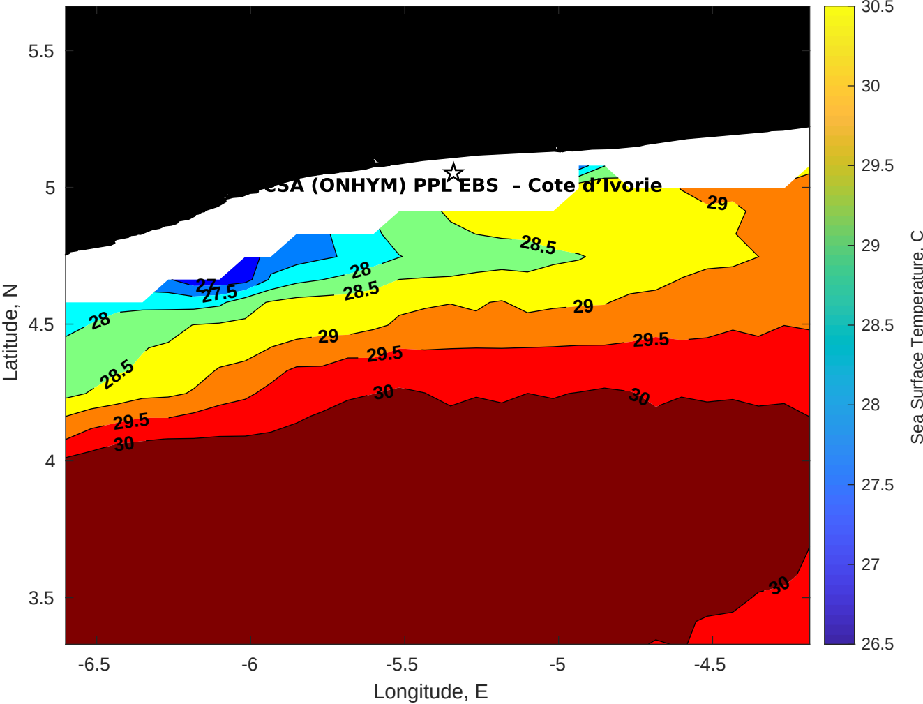
SST for CSA (ONHYM) PPL EBS - Cote d'Ivoire at 26-Apr-2025 00:00:00
