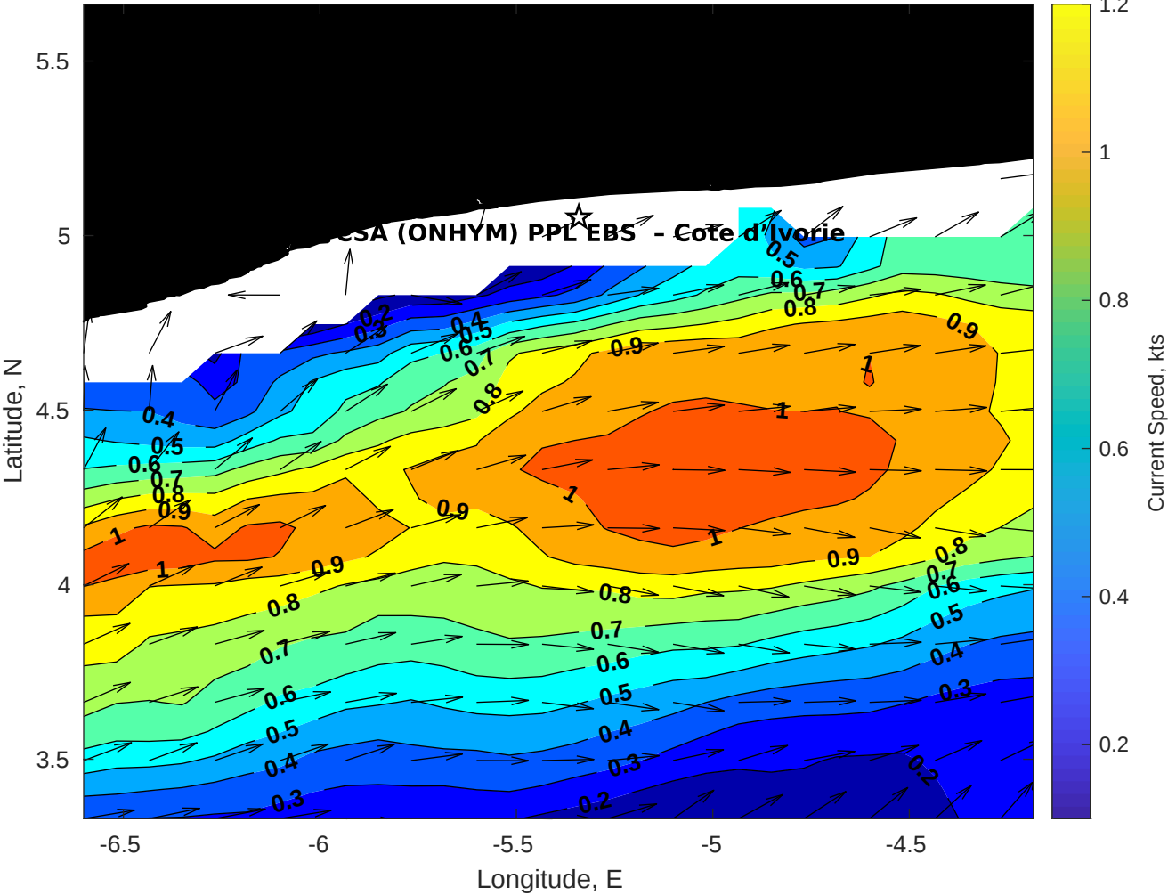
Surface Currents for CSA (ONHYM) PPL EBS - Cote d'Ivoire at 26-Apr-2025 00:00:00
