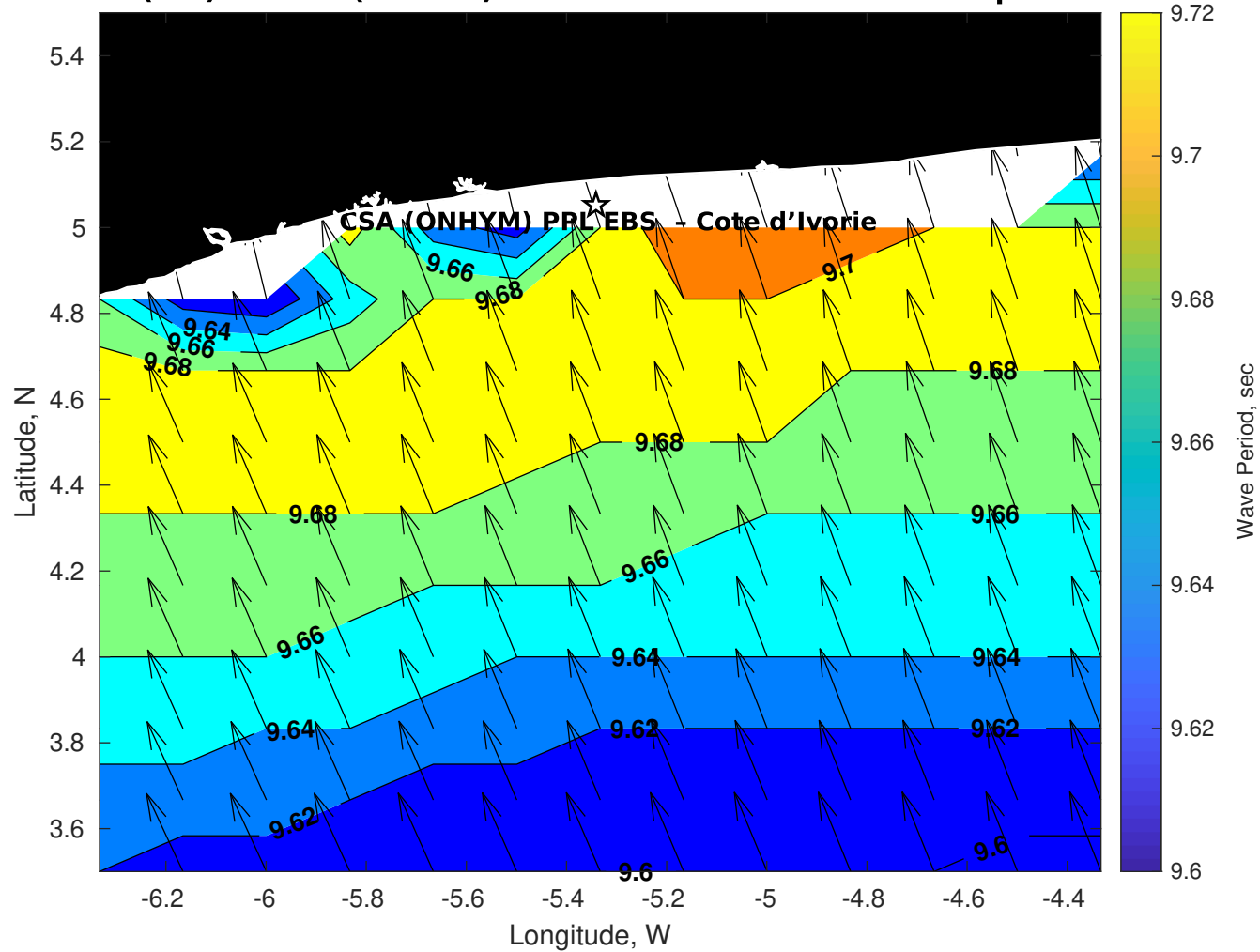
Wave Period (sec) for CSA (ONHYM) PPL EBS - Cote d'Ivoire at 27-Apr-2025 09:00:00
