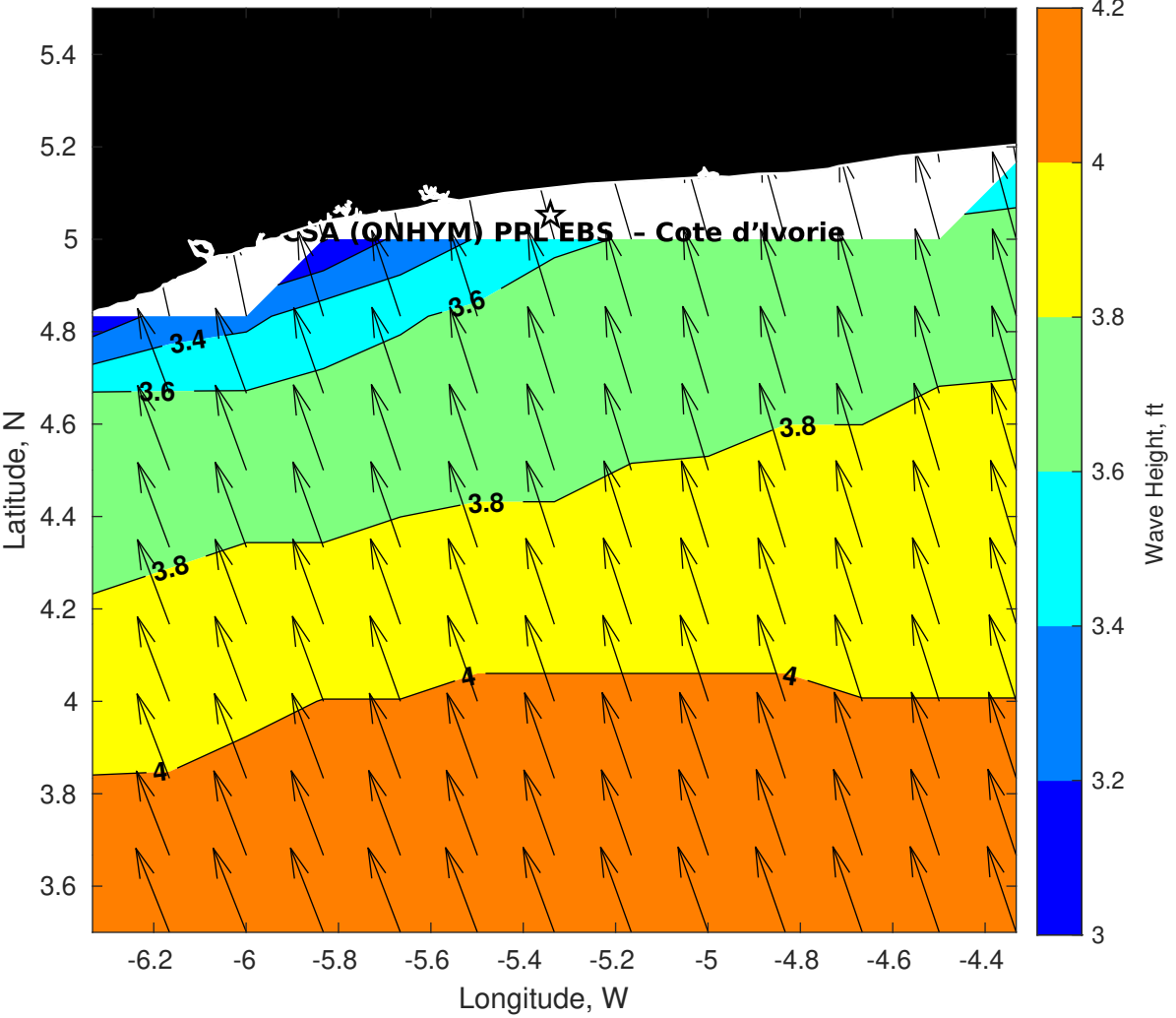
Wave Height (ft) for CSA (ONHYM) PPL EBS - Cote d'Ivoire at 27-Apr-2025 09:00:00
