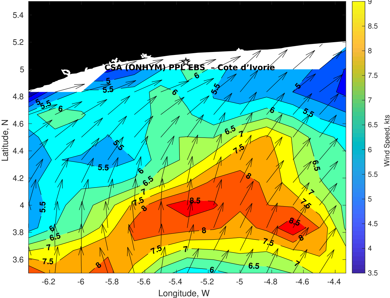
Winds (kts) for CSA (ONHYM) PPL EBS - Cote d'Ivoire at 27-Apr-2025 09:00:00
