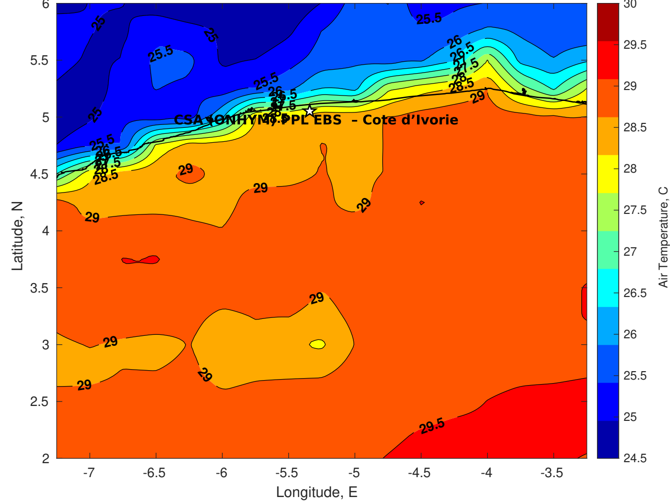
Air Temperature (C) for CSA (ONHYM) PPL EBS - Cote d'Ivoire at 27-Apr-2025
