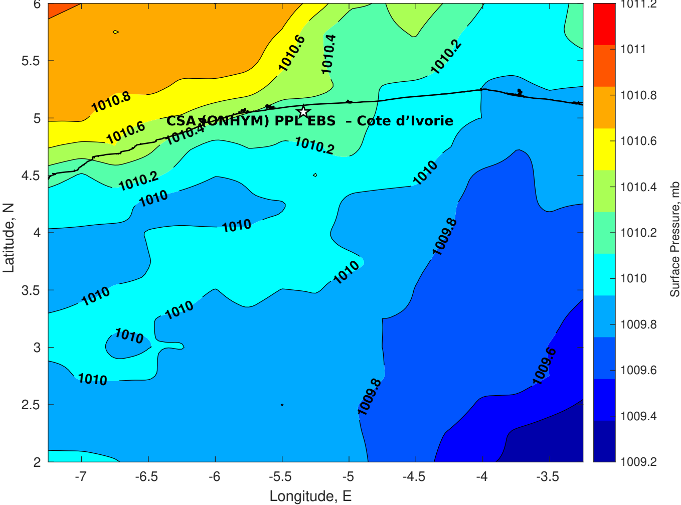
Surface Pressure (mb) for CSA (ONHYM) PPL EBS - Cote d'Ivoire at 27-Apr-2025 00:00:00
