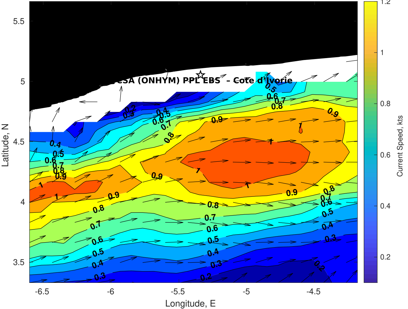
Surface Currents for CSA (ONHYM) PPL EBS - Cote d'Ivoire at 26-Apr-2025 00:00:00
