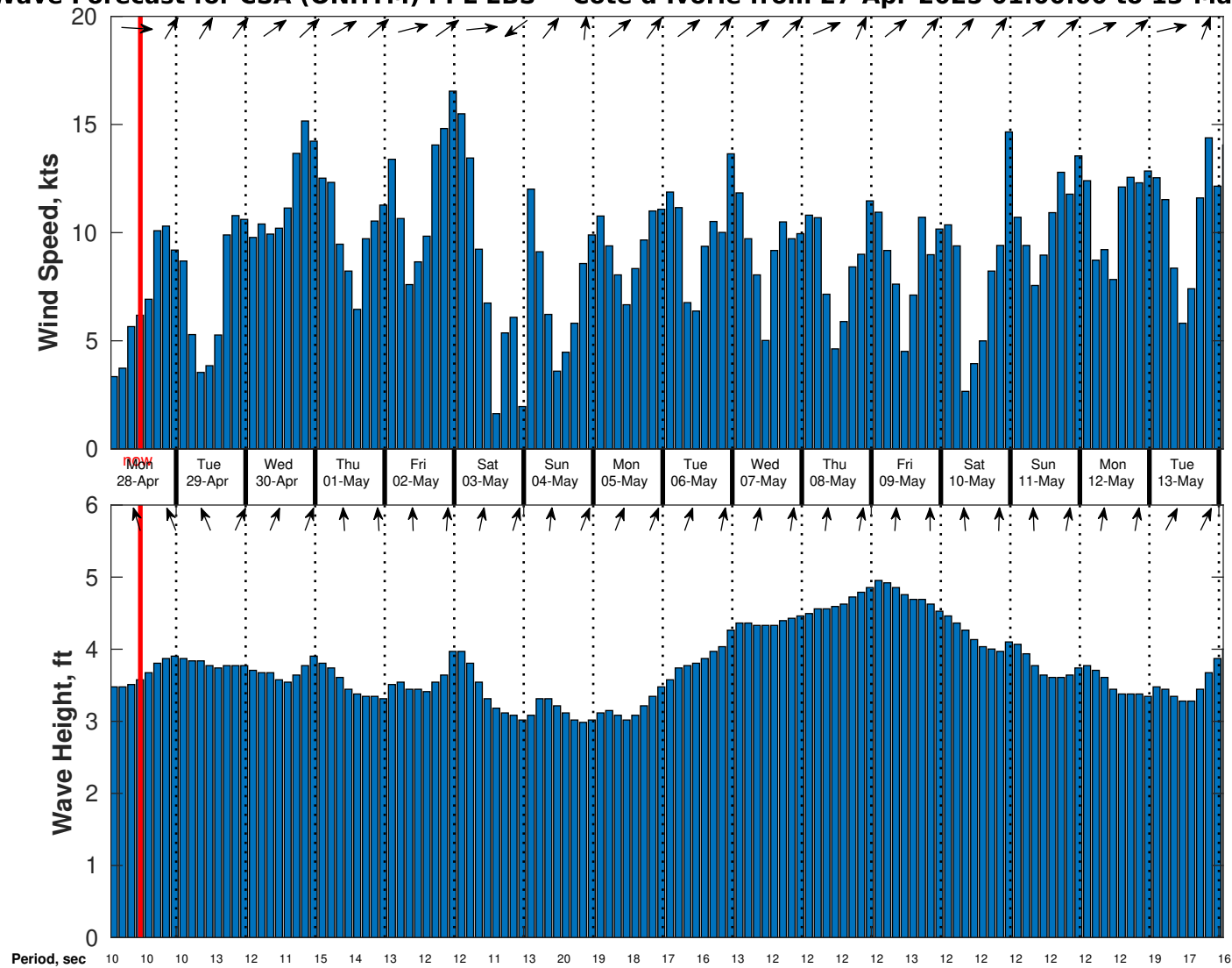
Wind & Wave Forecast for CSA (ONHYM) PPL EBS - Cote d'Ivoire from 27-Apr-2025 01:00:00 to 13-May-2025 01:00:00
