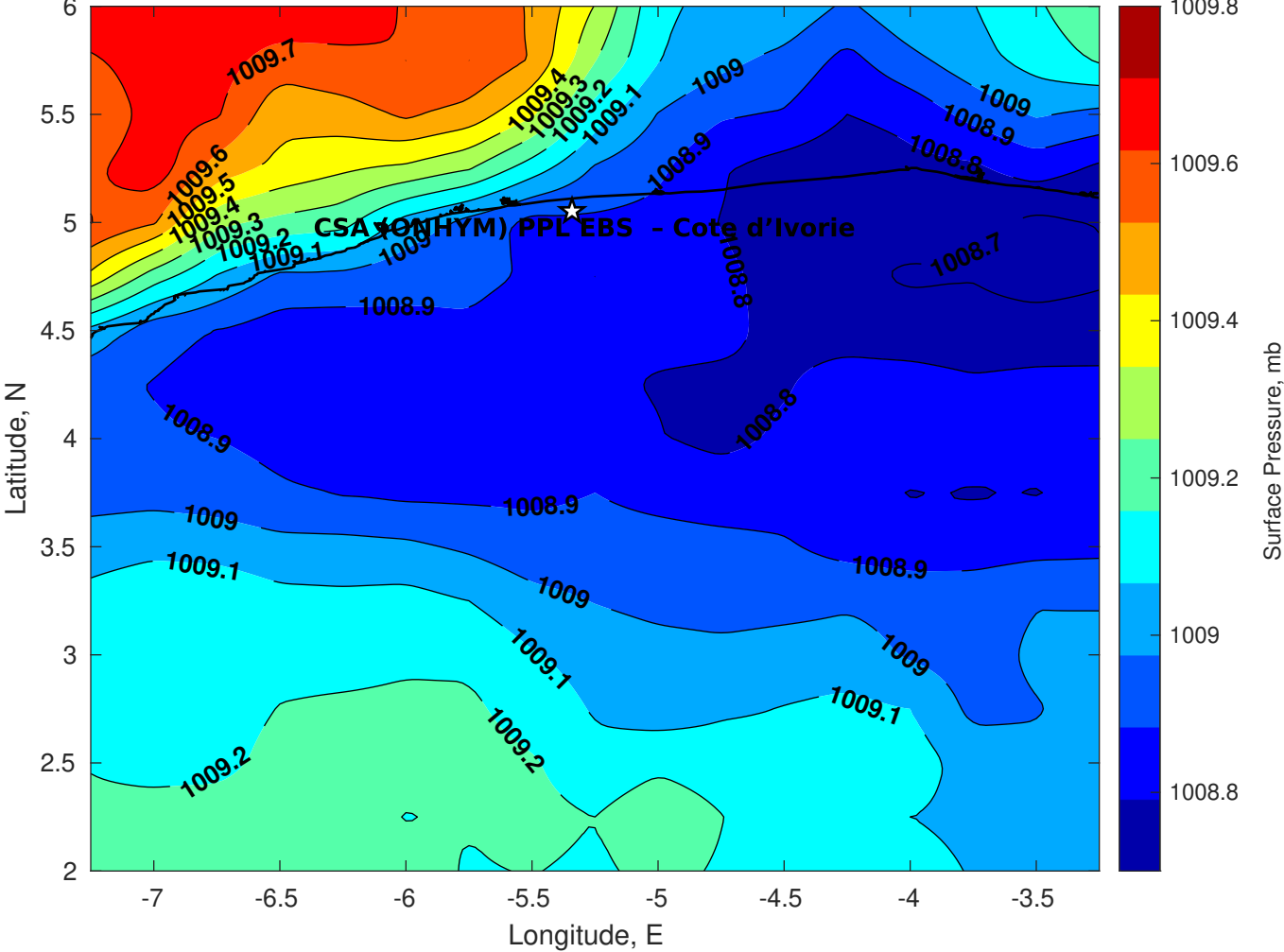
Surface Pressure (mb) for CSA (ONHYM) PPL EBS - Cote d'Ivoire at 29-Apr-2025 00:00:00
