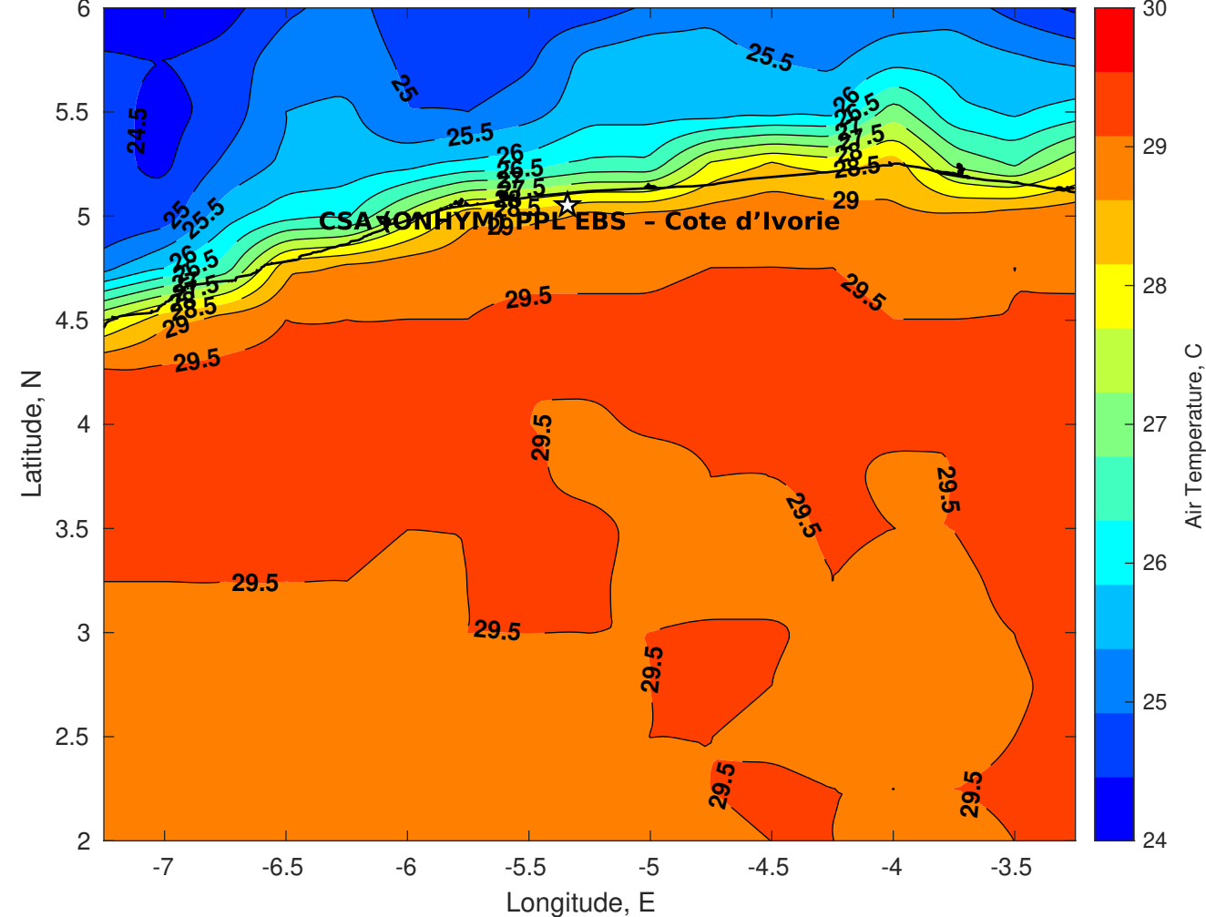
Air Temperature (C) for CSA (ONHYM) PPL EBS - Cote d'Ivoire at 27-Apr-2025
