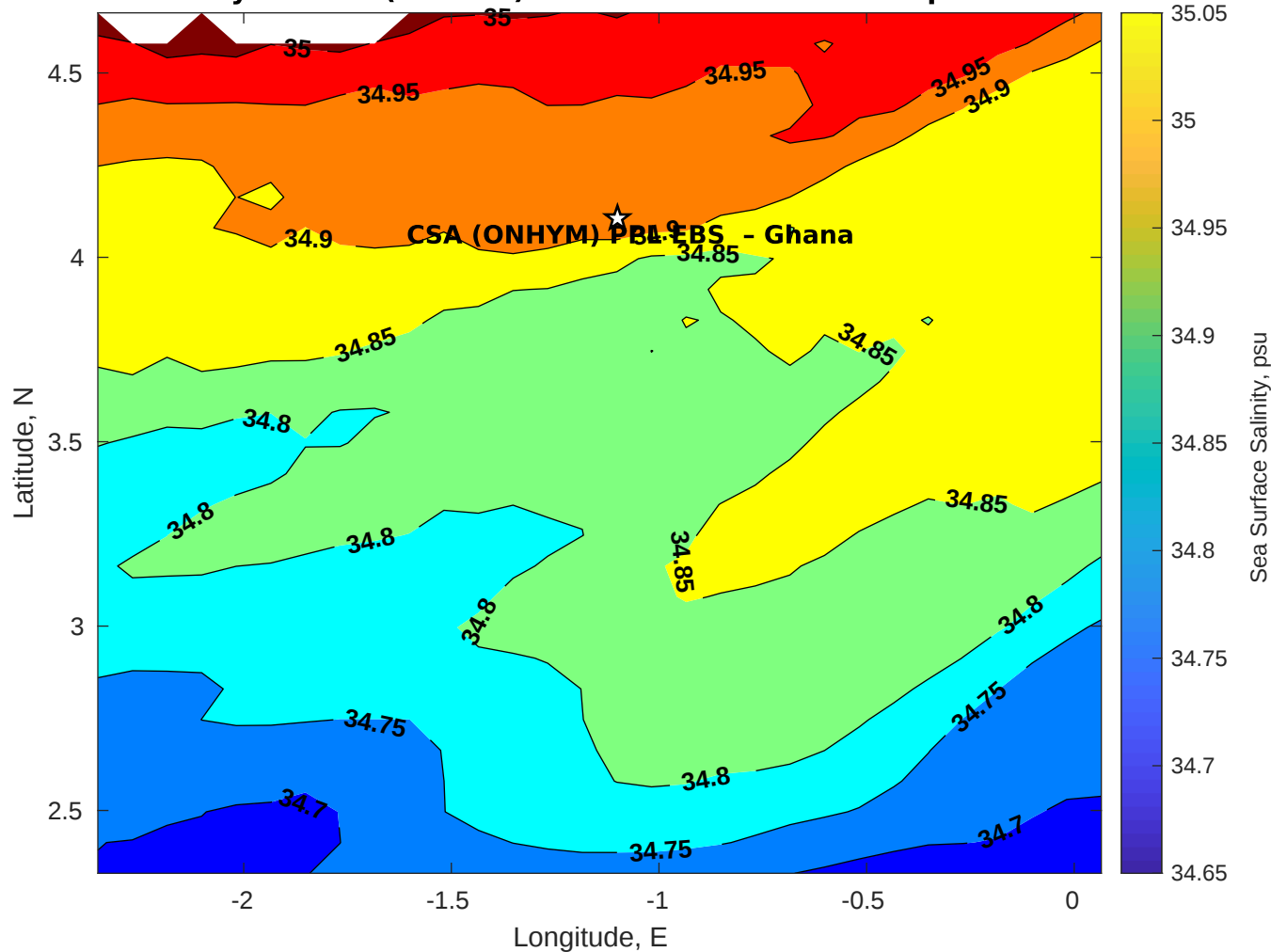
Surface Salinity for CSA (ONHYM) PPL EBS - Ghana at 26-Apr-2025 00:00:00
