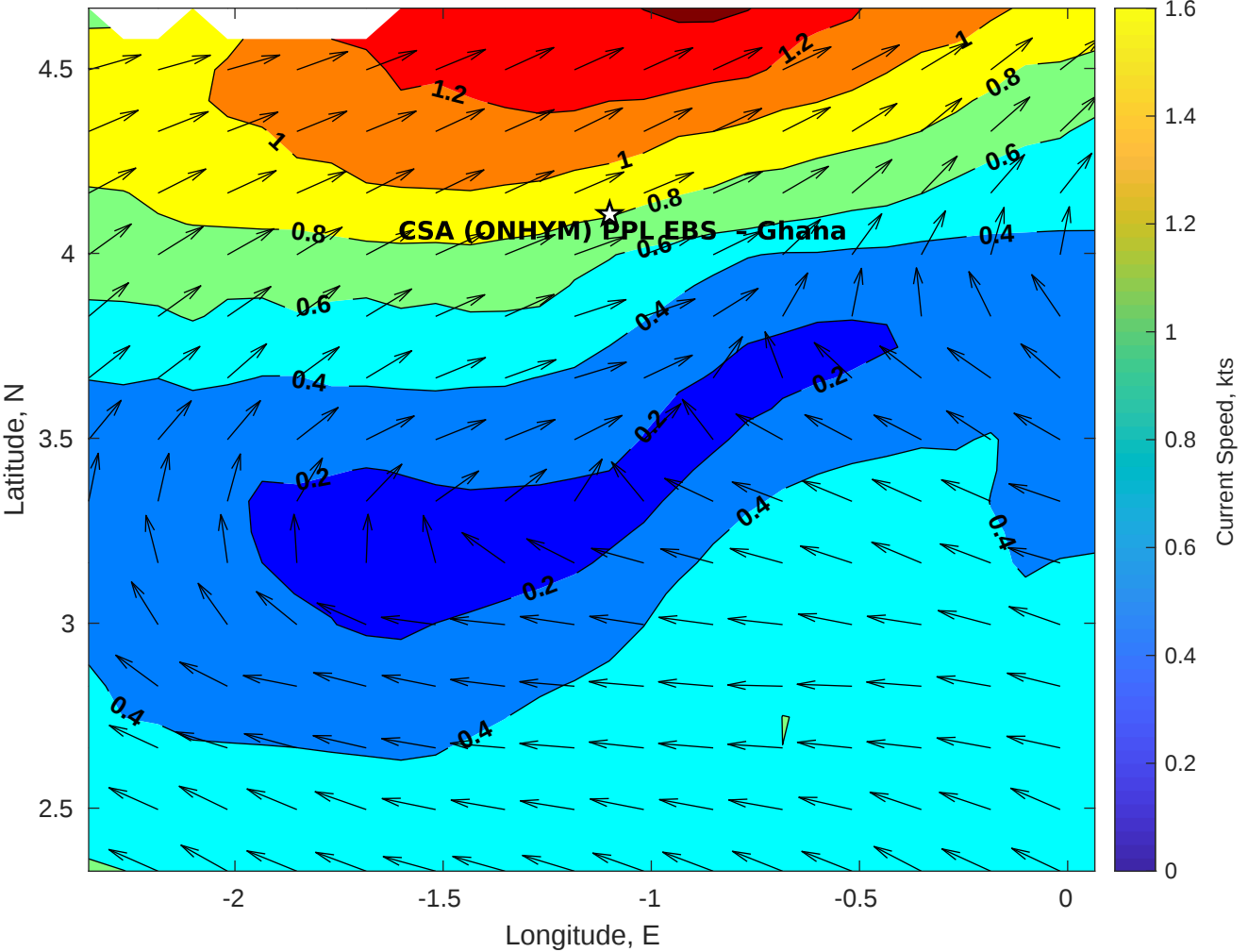
Surface Currents for CSA (ONHYM) PPL EBS - Ghana at 26-Apr-2025 00:00:00
