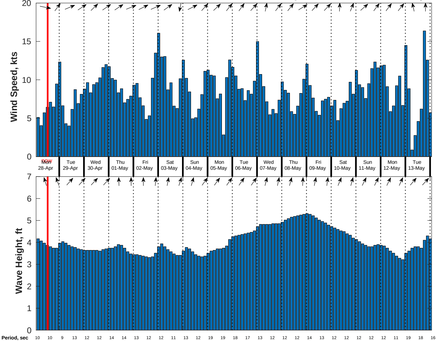
Wind & Wave Forecast for CSA (ONHYM) PPL EBS - Ghana from 27-Apr-2025 02:00:00 to 13-May-2025 02:00:00
