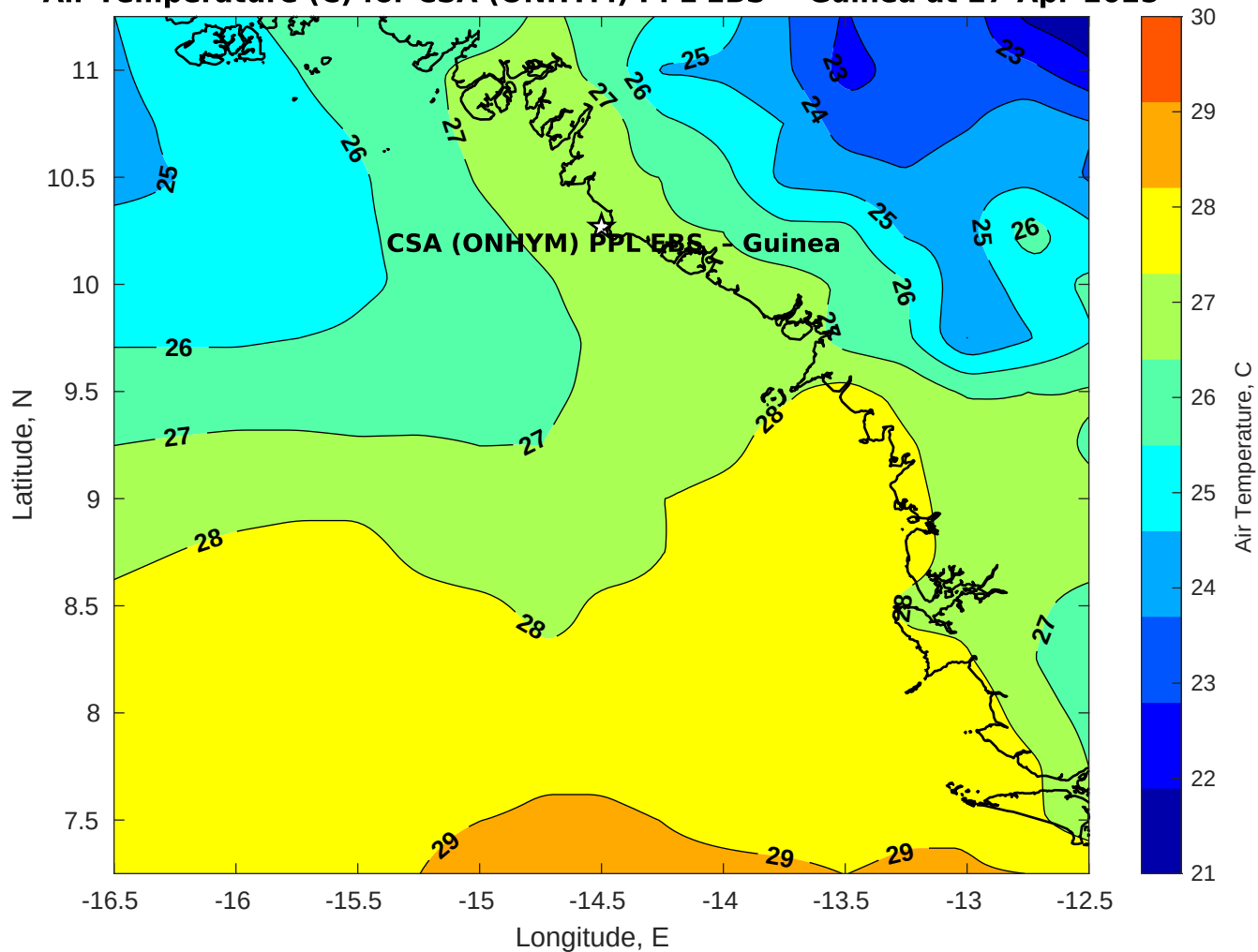
Air Temperature (C) for CSA (ONHYM) PPL EBS - Guinea at 27-Apr-2025
