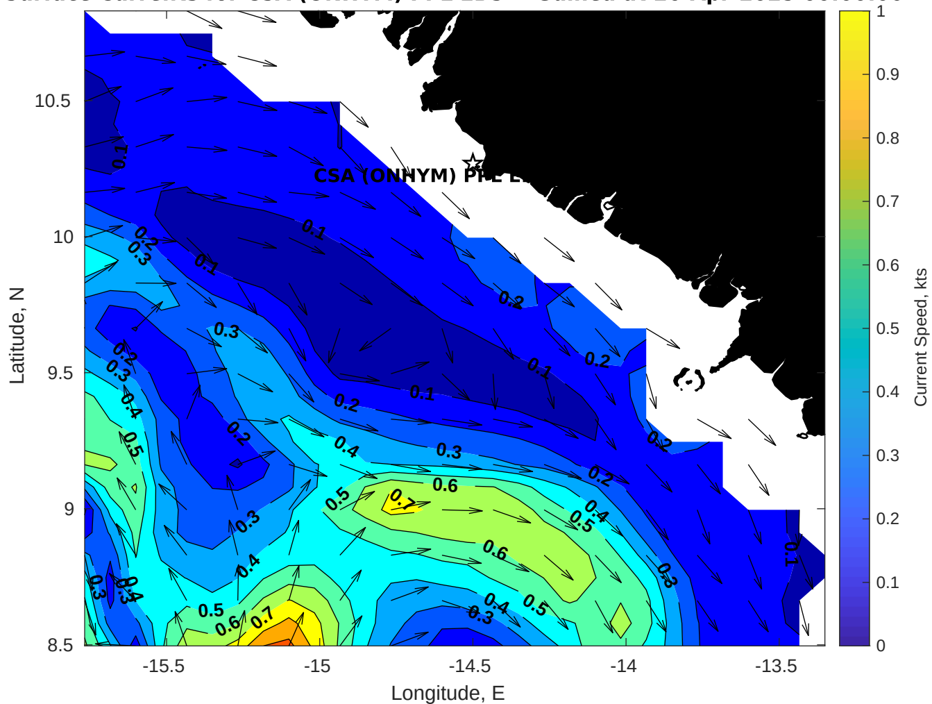
Surface Currents for CSA (ONHYM) PPL EBS - Guinea at 26-Apr-2025 00:00:00
