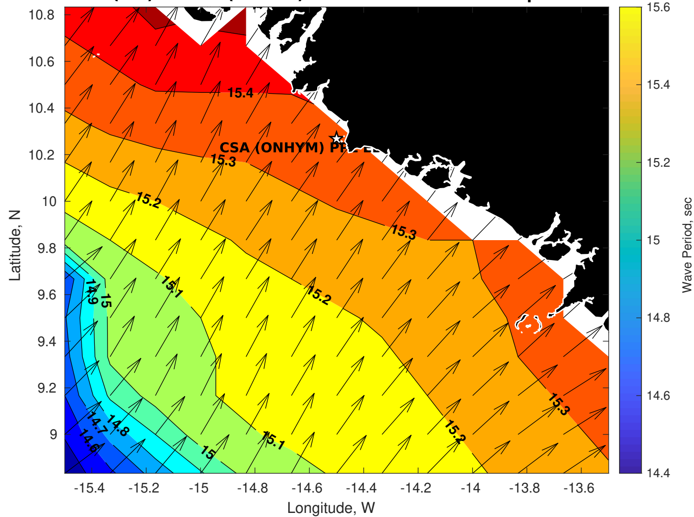
Wave Period (sec) for CSA (ONHYM) PPL EBS - Guinea at 27-Apr-2025 09:00:00
