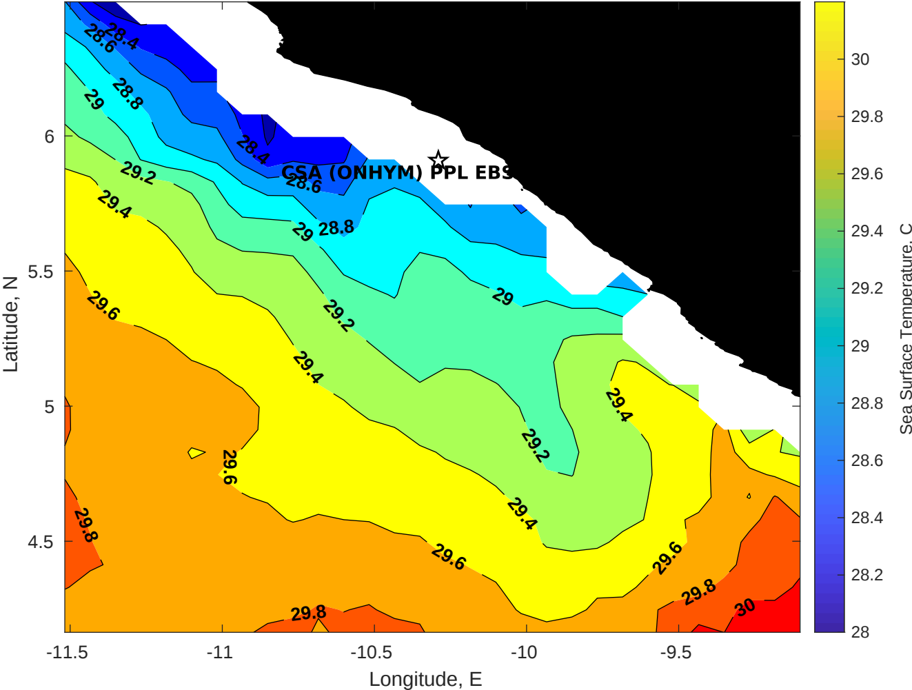
SST for CSA (ONHYM) PPL EBS - Liberia at 26-Apr-2025 00:00:00
