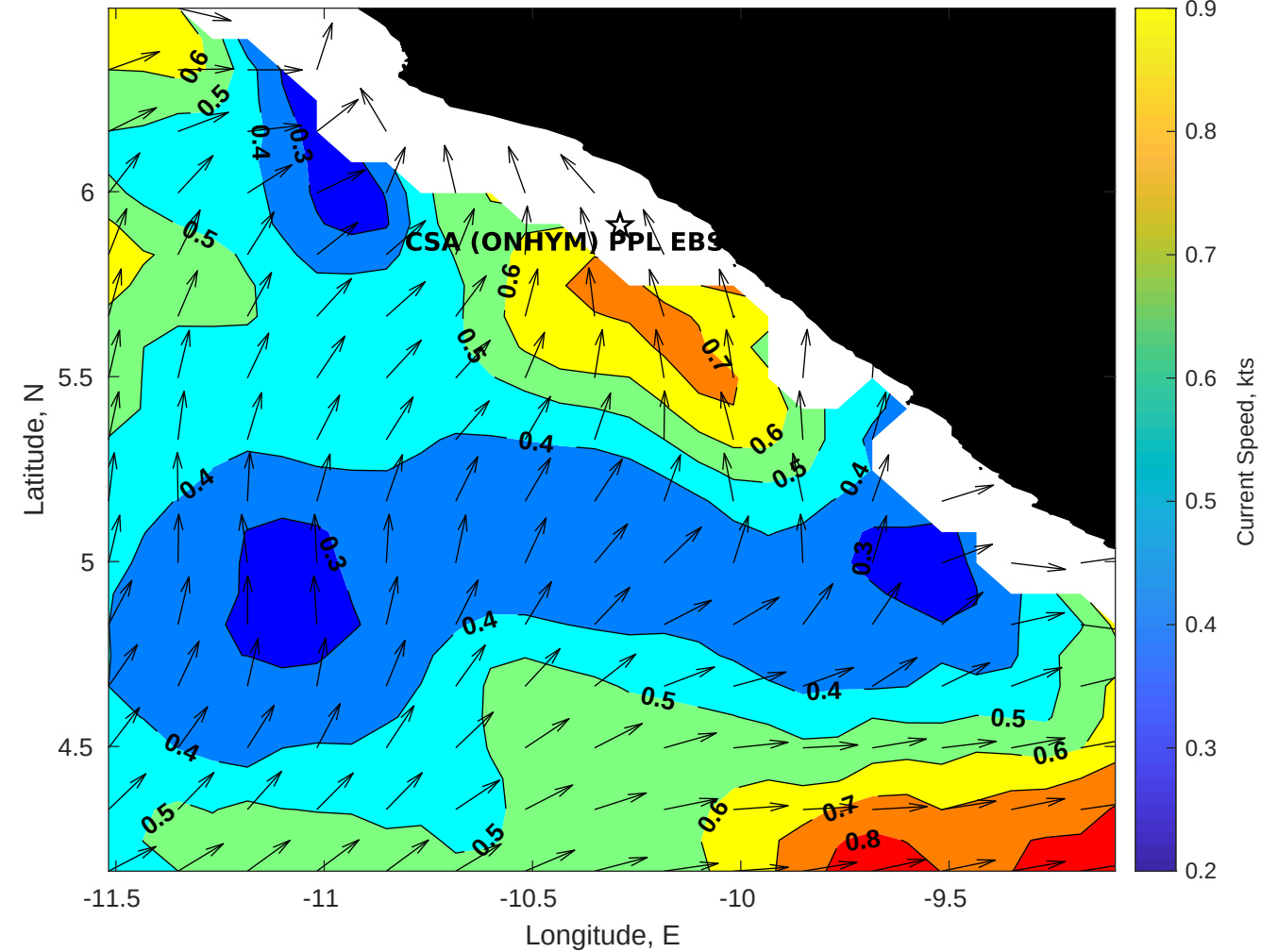
Surface Currents for CSA (ONHYM) PPL EBS - Liberia at 26-Apr-2025 00:00:00
