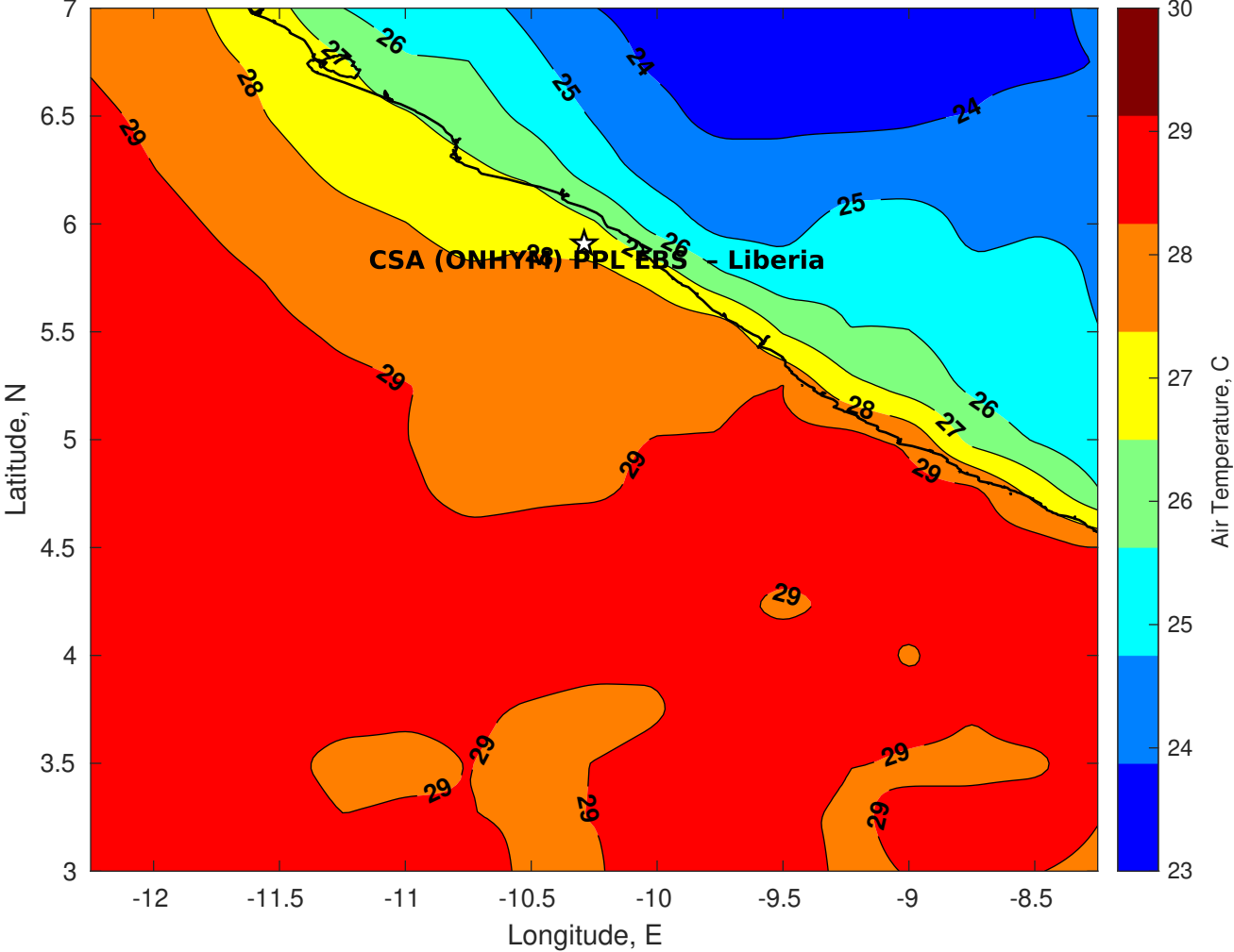
Air Temperature (C) for CSA (ONHYM) PPL EBS - Liberia at 27-Apr-2025
