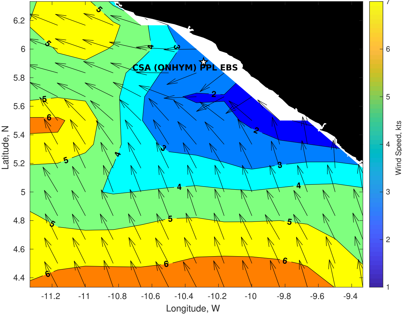
Winds (kts) for CSA (ONHYM) PPL EBS - Liberia at 27-Apr-2025 09:00:00
