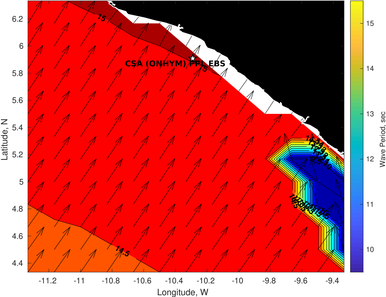
Wave Period (sec) for CSA (ONHYM) PPL EBS - Liberia at 27-Apr-2025 09:00:00
