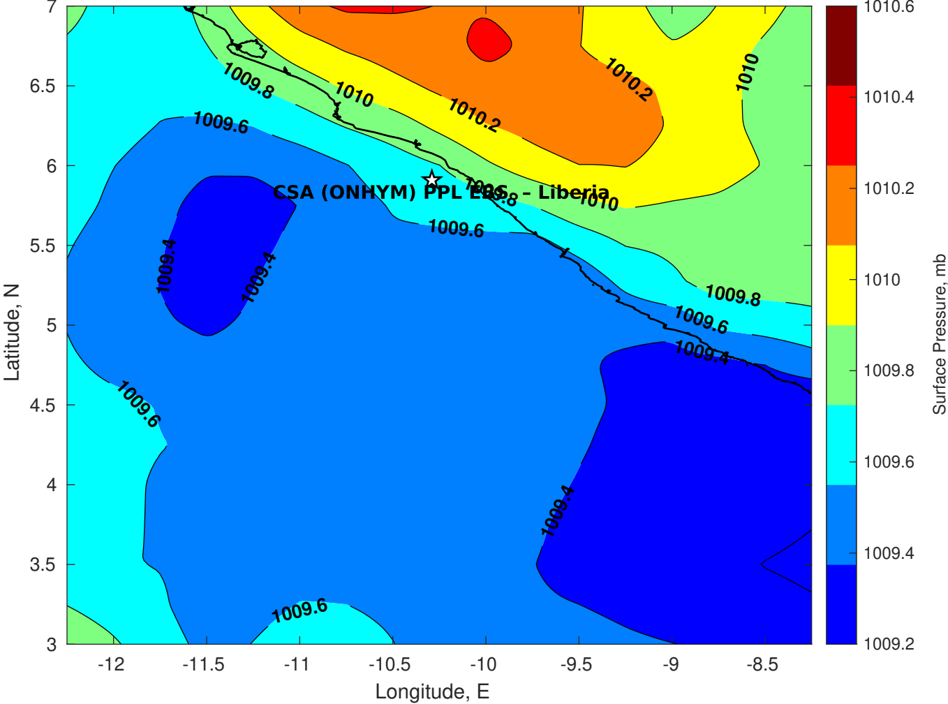
Surface Pressure (mb) for CSA (ONHYM) PPL EBS - Liberia at 29-Apr-2025 00:00:00
