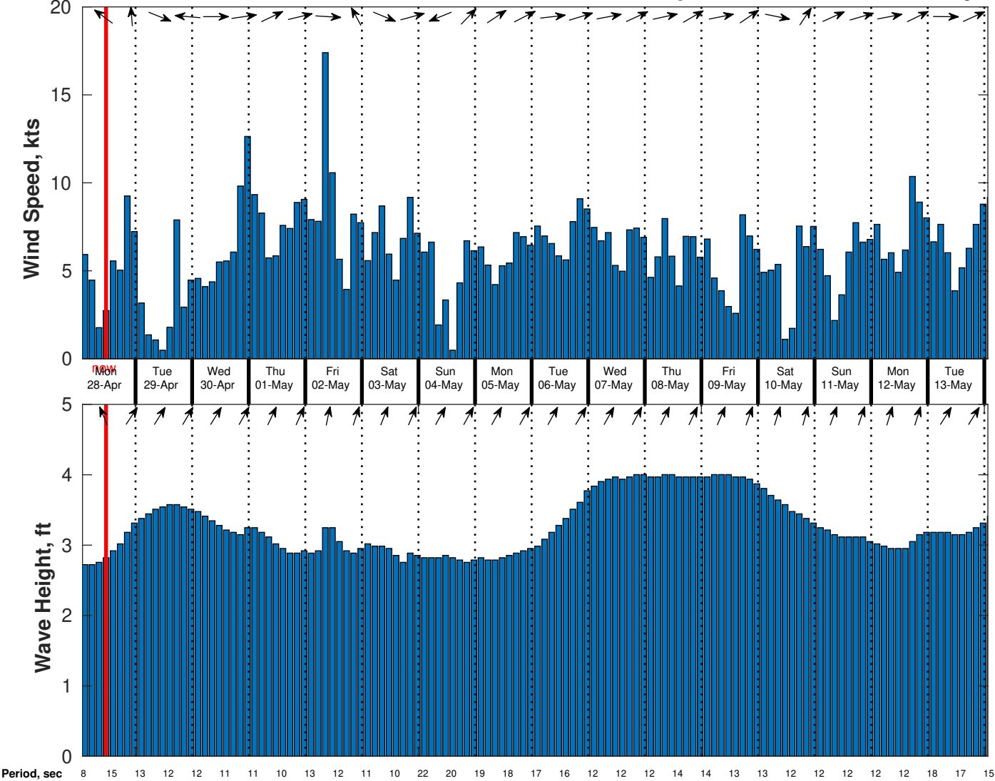
Wind & Wave Forecast for CSA (ONHYM) PPL EBS - Liberia from 27-Apr-2025 01:00:00 to 13-May-2025 01:00:00
