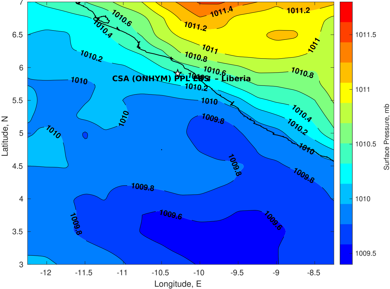
Surface Pressure (mb) for CSA (ONHYM) PPL EBS - Liberia at 28-Apr-2025 00:00:00
