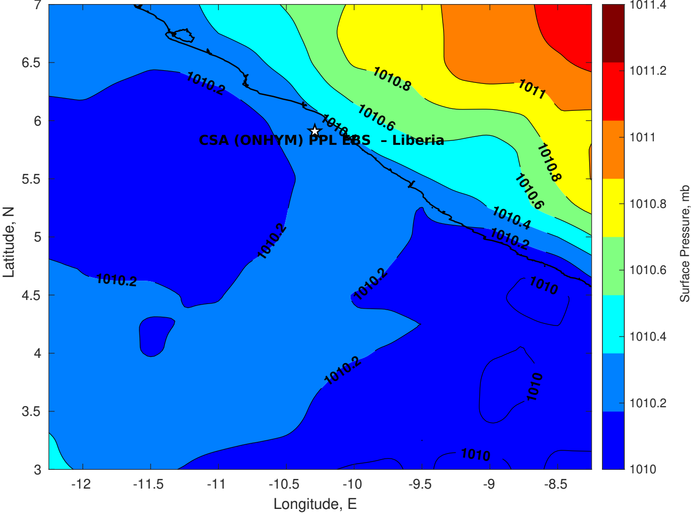
Surface Pressure (mb) for CSA (ONHYM) PPL EBS - Liberia at 27-Apr-2025 00:00:00
