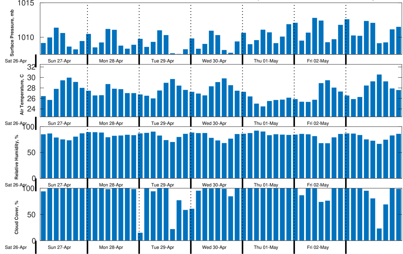
Met Forecast for CSA (ONHYM) PPL EBS - Liberia from 27-Apr-2025 00:00:00 to 04-May-2025 00:00:00
