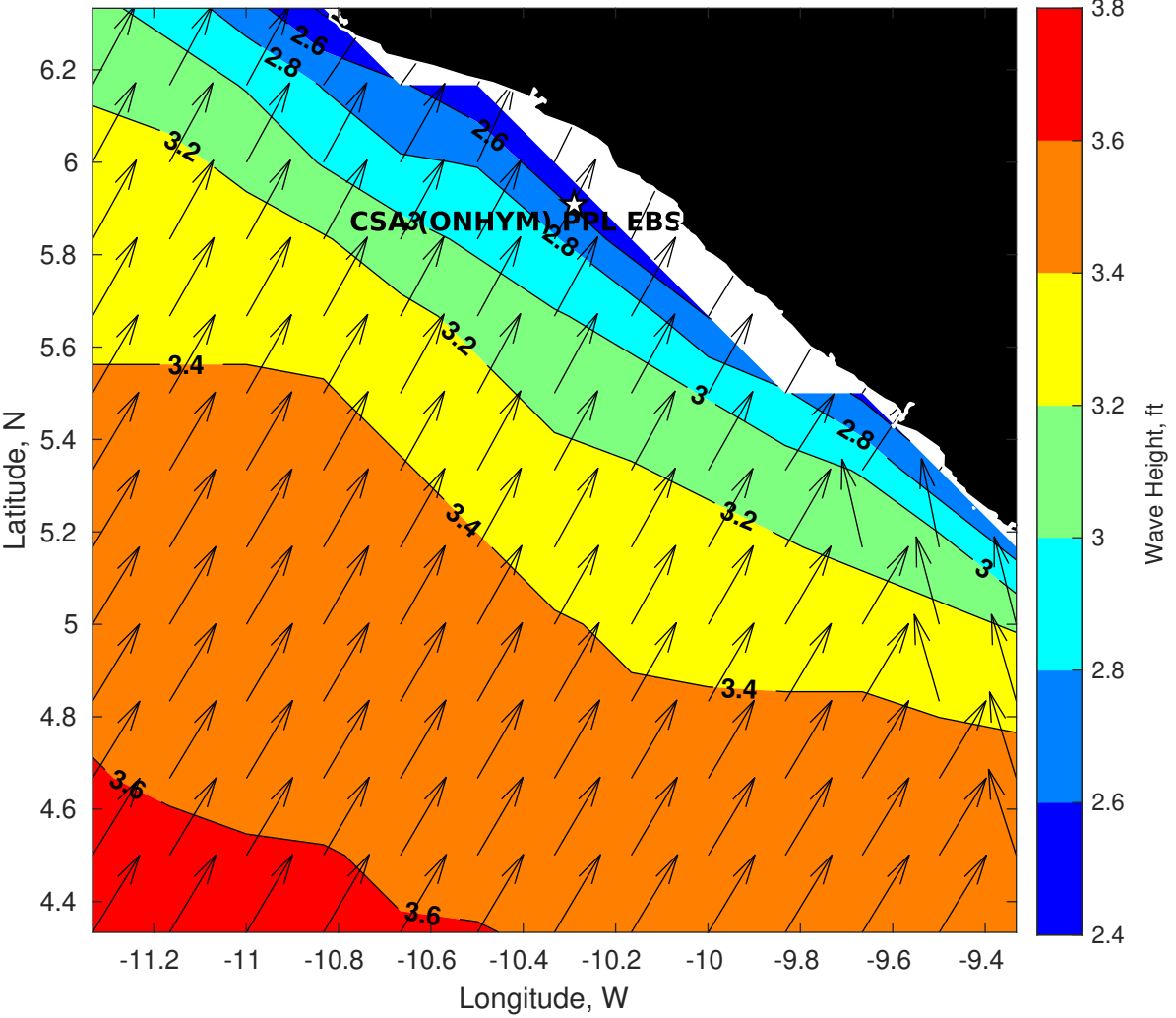
Wave Height (ft) for CSA (ONHYM) PPL EBS - Liberia at 27-Apr-2025 09:00:00
