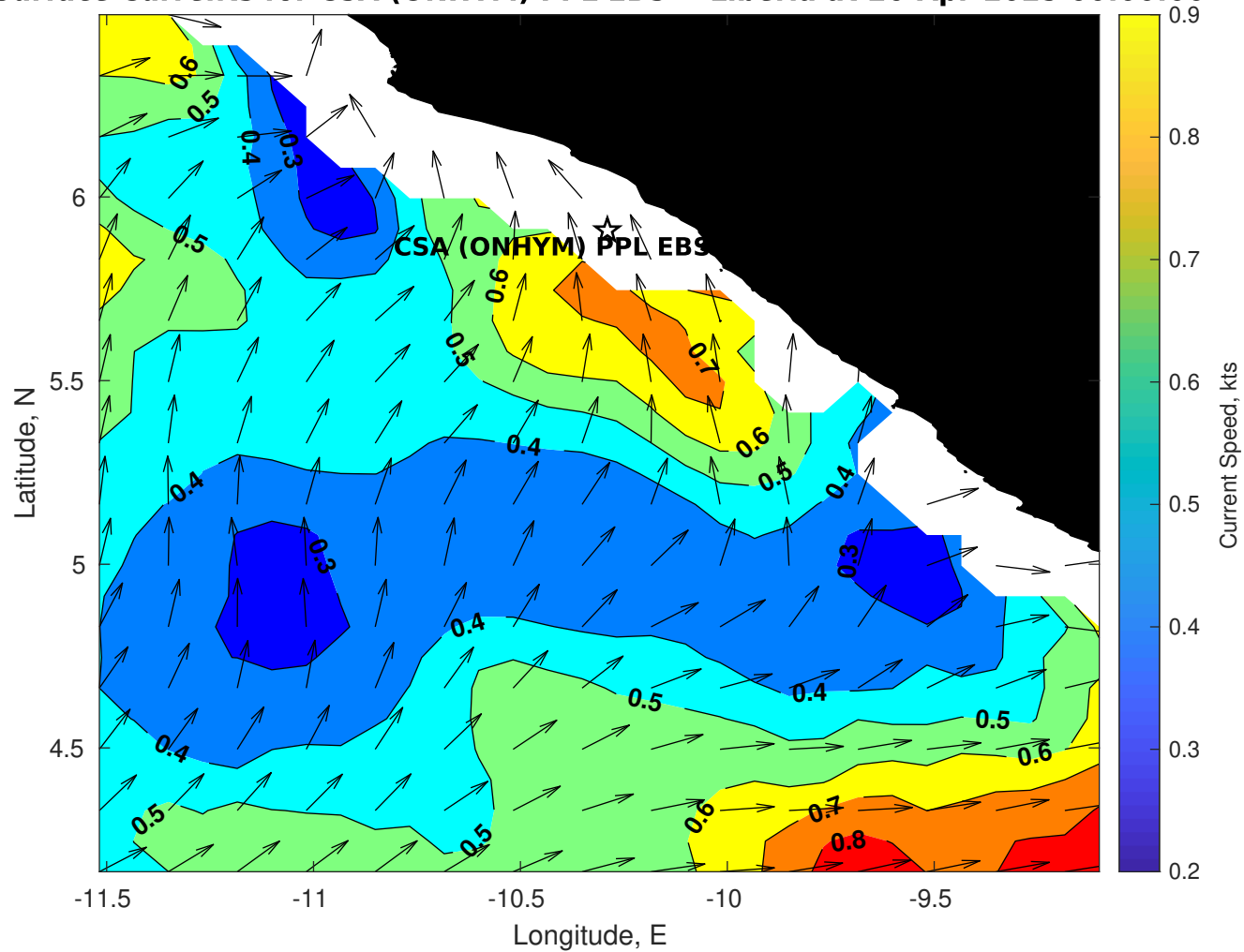
Surface Currents for CSA (ONHYM) PPL EBS - Liberia at 26-Apr-2025 00:00:00
