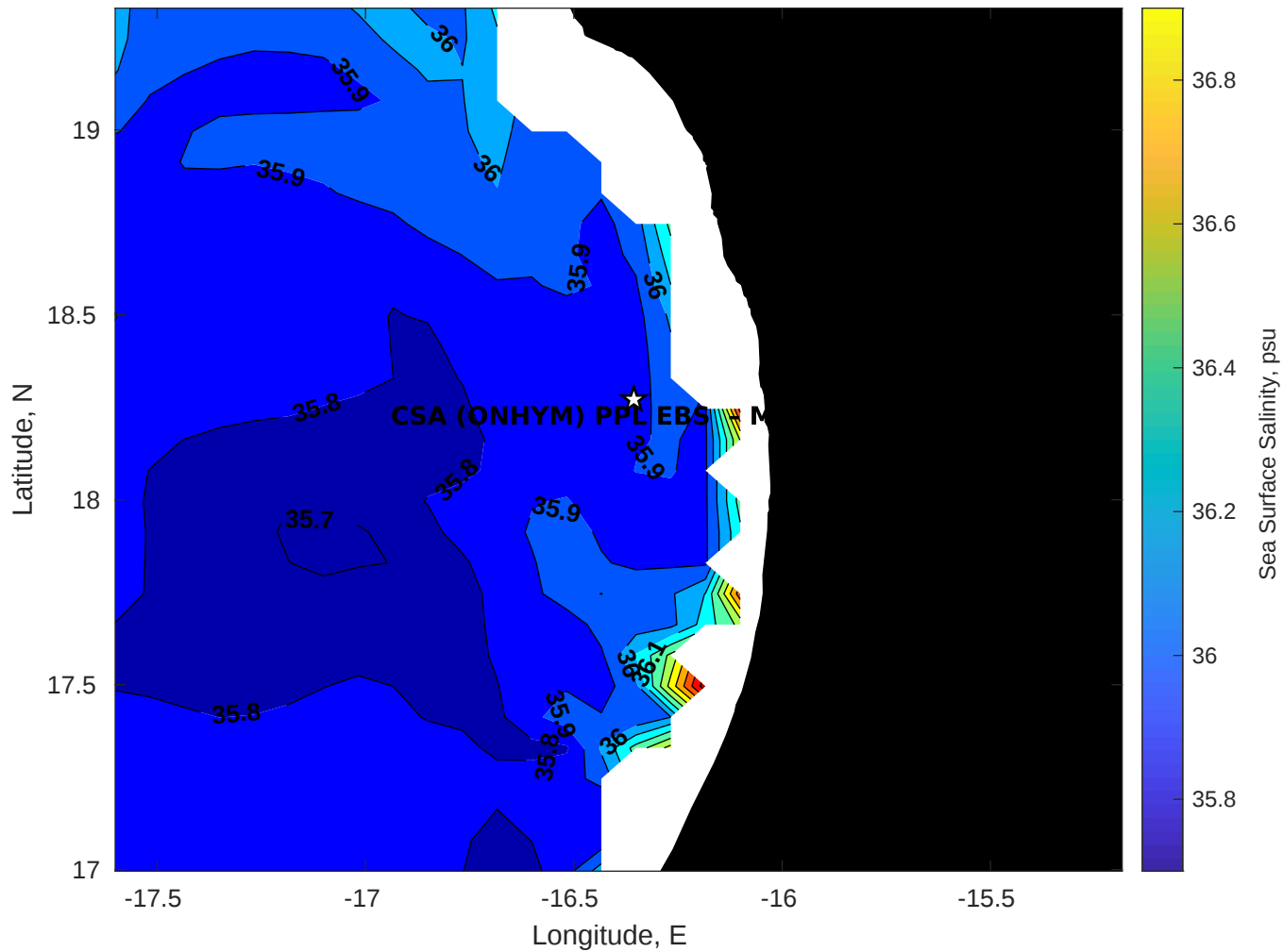
Surface Salinity for CSA (ONHYM) PPL EBS - Mauritania at 26-Apr-2025 00:00:00
