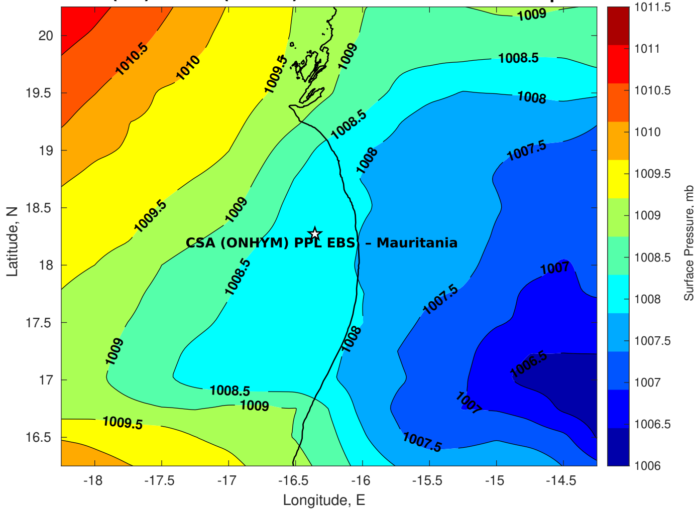
Surface Pressure (mb) for CSA (ONHYM) PPL EBS - Mauritania at 27-Apr-2025 00:00:00
