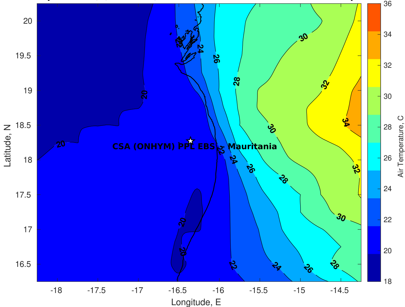
Air Temperature (C) for CSA (ONHYM) PPL EBS - Mauritania at 27-Apr-2025
