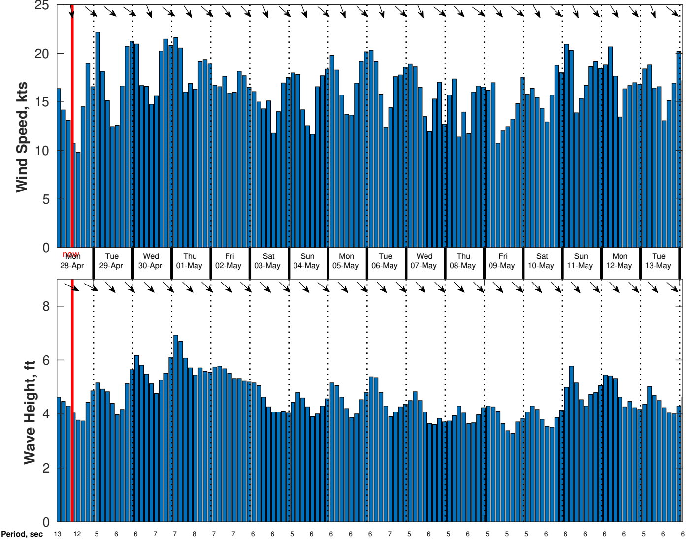
Wind & Wave Forecast for CSA (ONHYM) PPL EBS - Mauritania from 27-Apr-2025 01:00:00 to 13-May-2025 01:00:00
