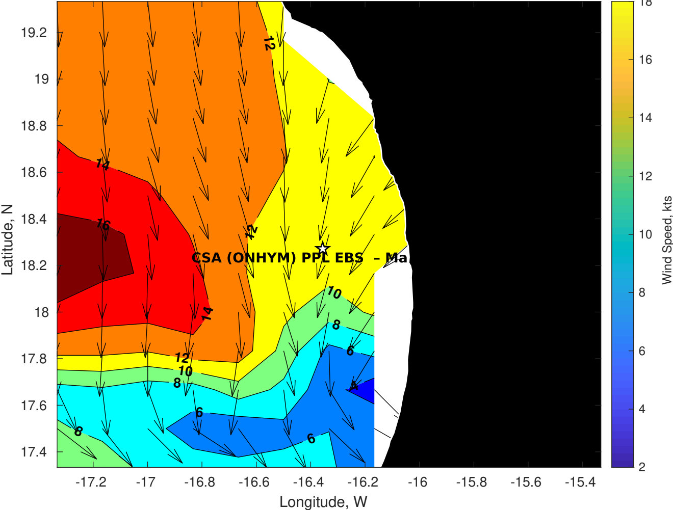
Winds (kts) for CSA (ONHYM) PPL EBS - Mauritania at 27-Apr-2025 09:00:00
