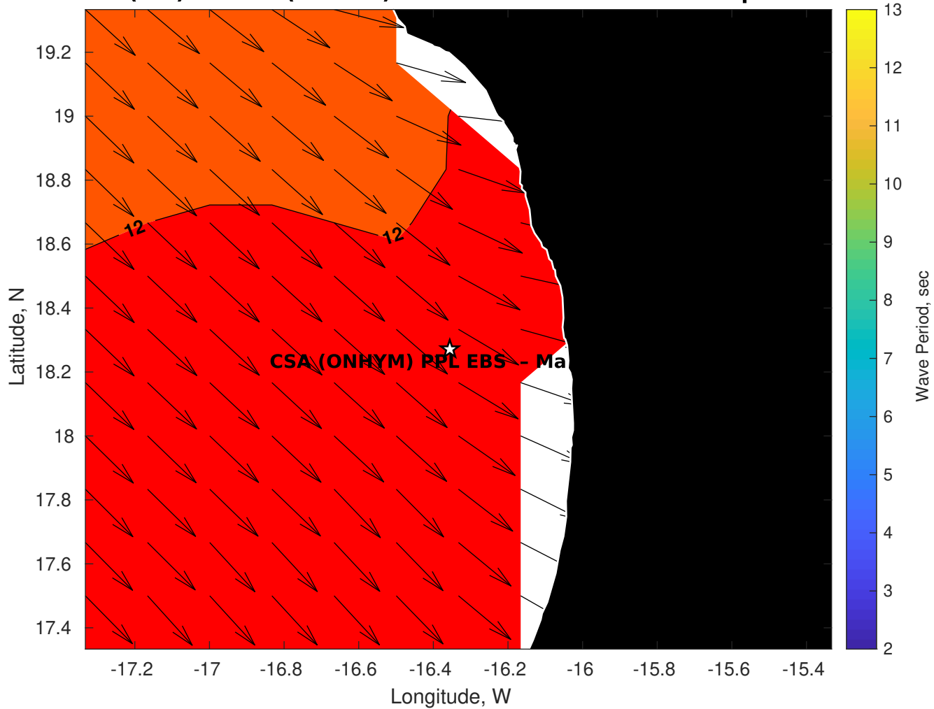
Wave Period (sec) for CSA (ONHYM) PPL EBS - Mauritania at 27-Apr-2025 09:00:00
