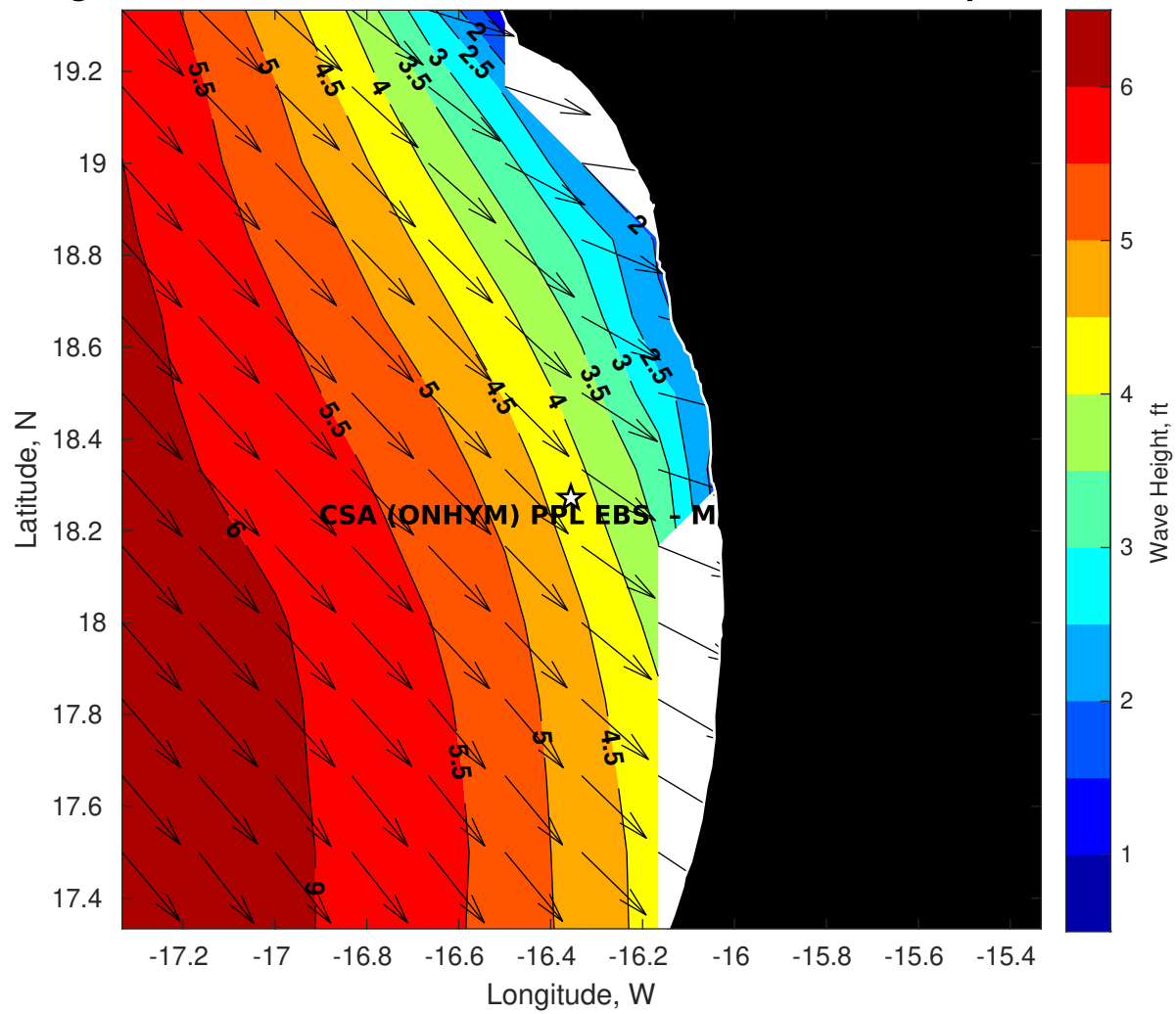
Wave Height (ft) for CSA (ONHYM) PPL EBS - Mauritania at 27-Apr-2025 09:00:00
