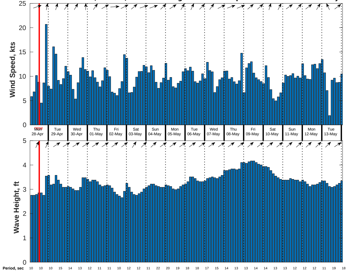
Wind & Wave Forecast for CSA (ONHYM) PPL EBS - Nigeria from 27-Apr-2025 02:00:00 to 13-May-2025 02:00:00
