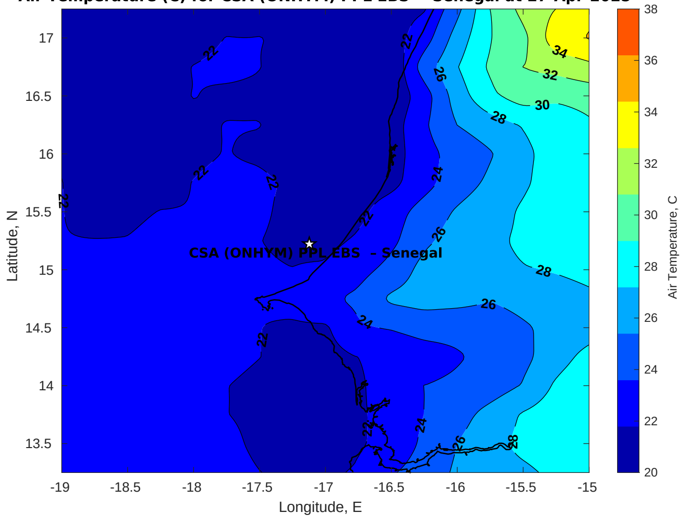
Air Temperature (C) for CSA (ONHYM) PPL EBS - Senegal at 27-Apr-2025
