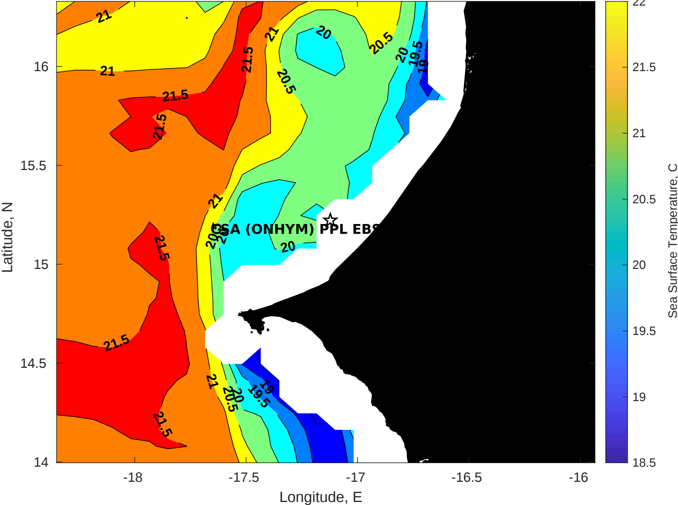
SST for CSA (ONHYM) PPL EBS - Senegal at 26-Apr-2025 00:00:00
