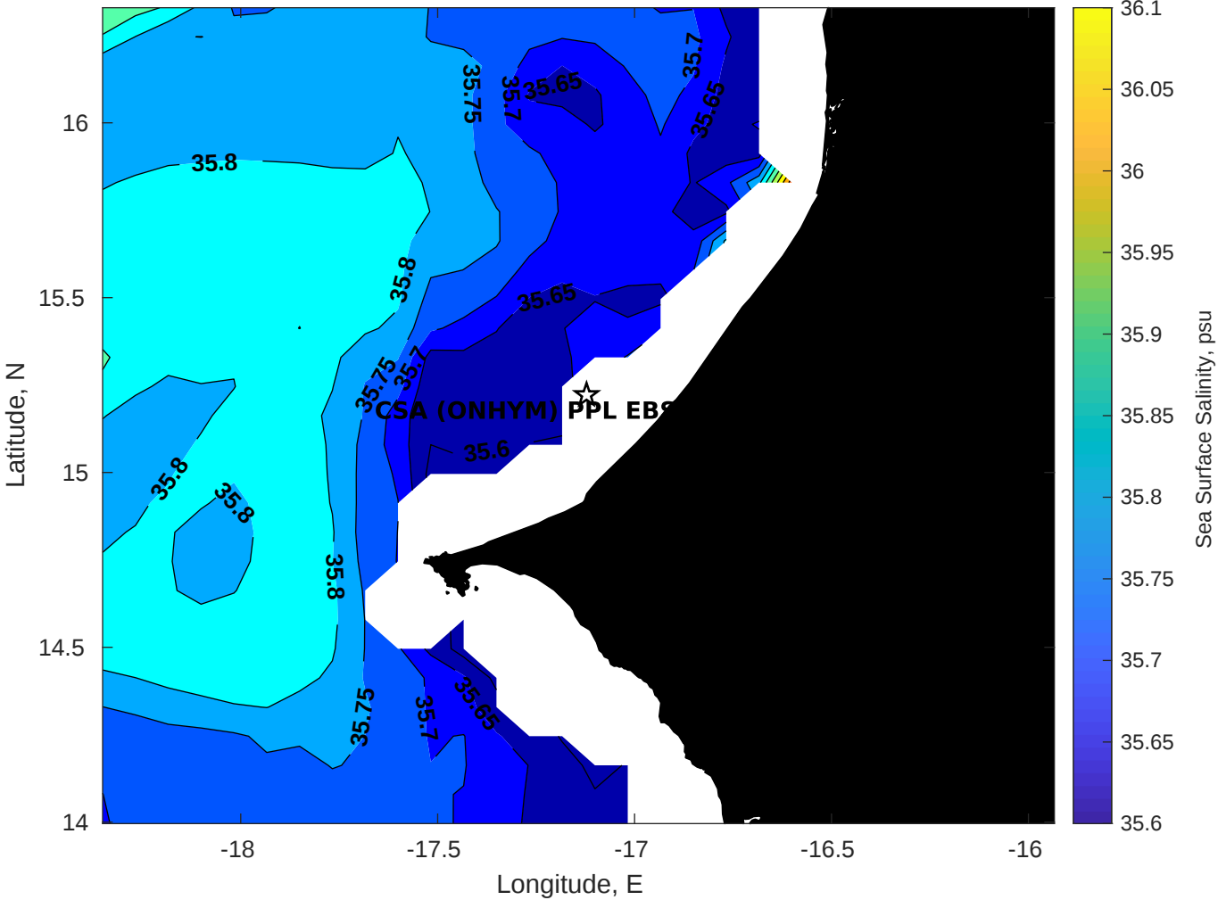
Surface Salinity for CSA (ONHYM) PPL EBS - Senegal at 26-Apr-2025 00:00:00
