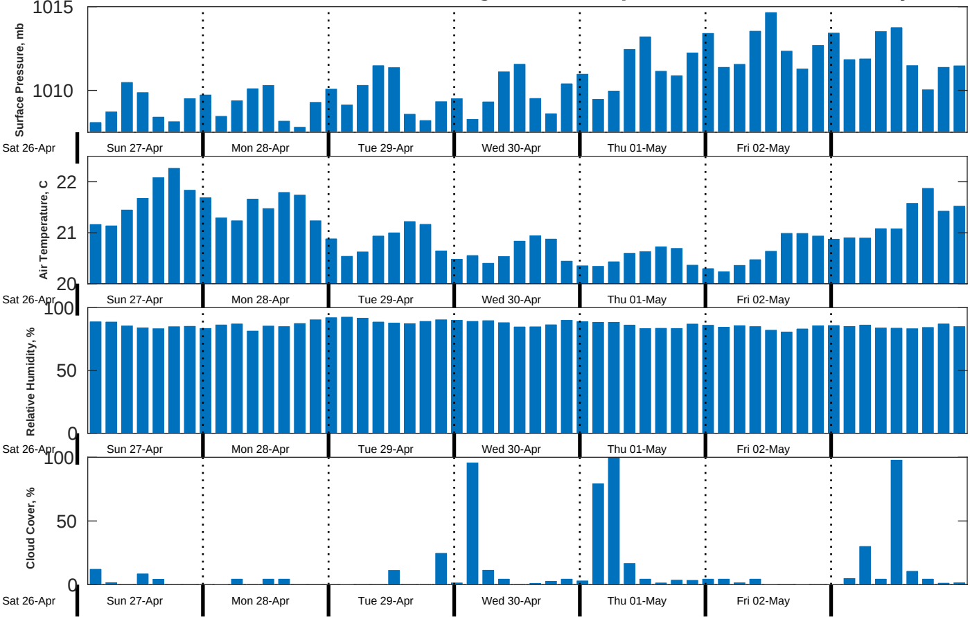
Met Forecast for CSA (ONHYM) PPL EBS - Senegal from 27-Apr-2025 00:00:00 to 04-May-2025 00:00:00
