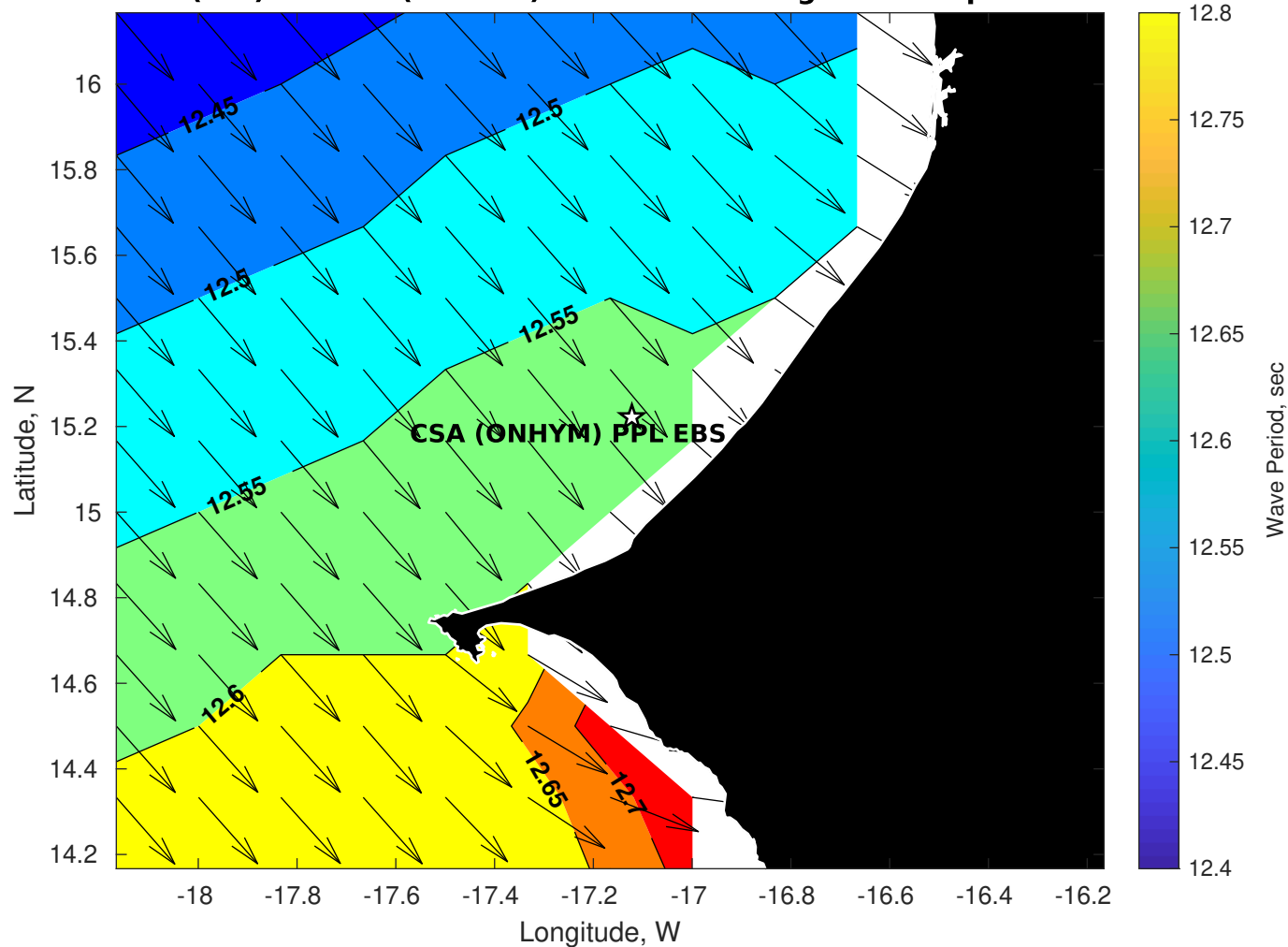
Wave Period (sec) for CSA (ONHYM) PPL EBS - Senegal at 27-Apr-2025 09:00:00
