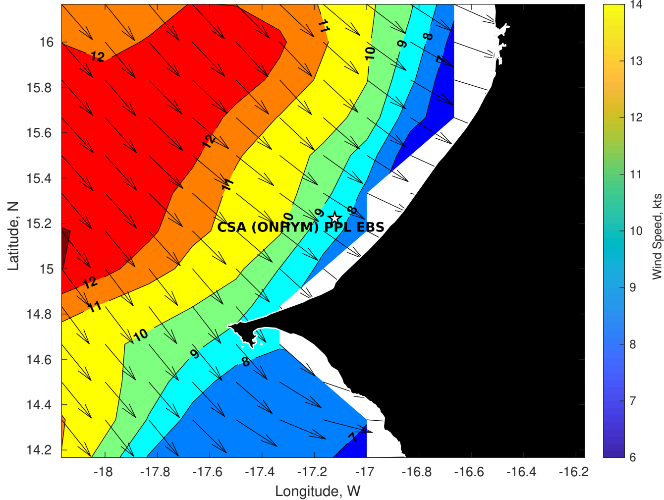
Winds (kts) for CSA (ONHYM) PPL EBS - Senegal at 27-Apr-2025 09:00:00
