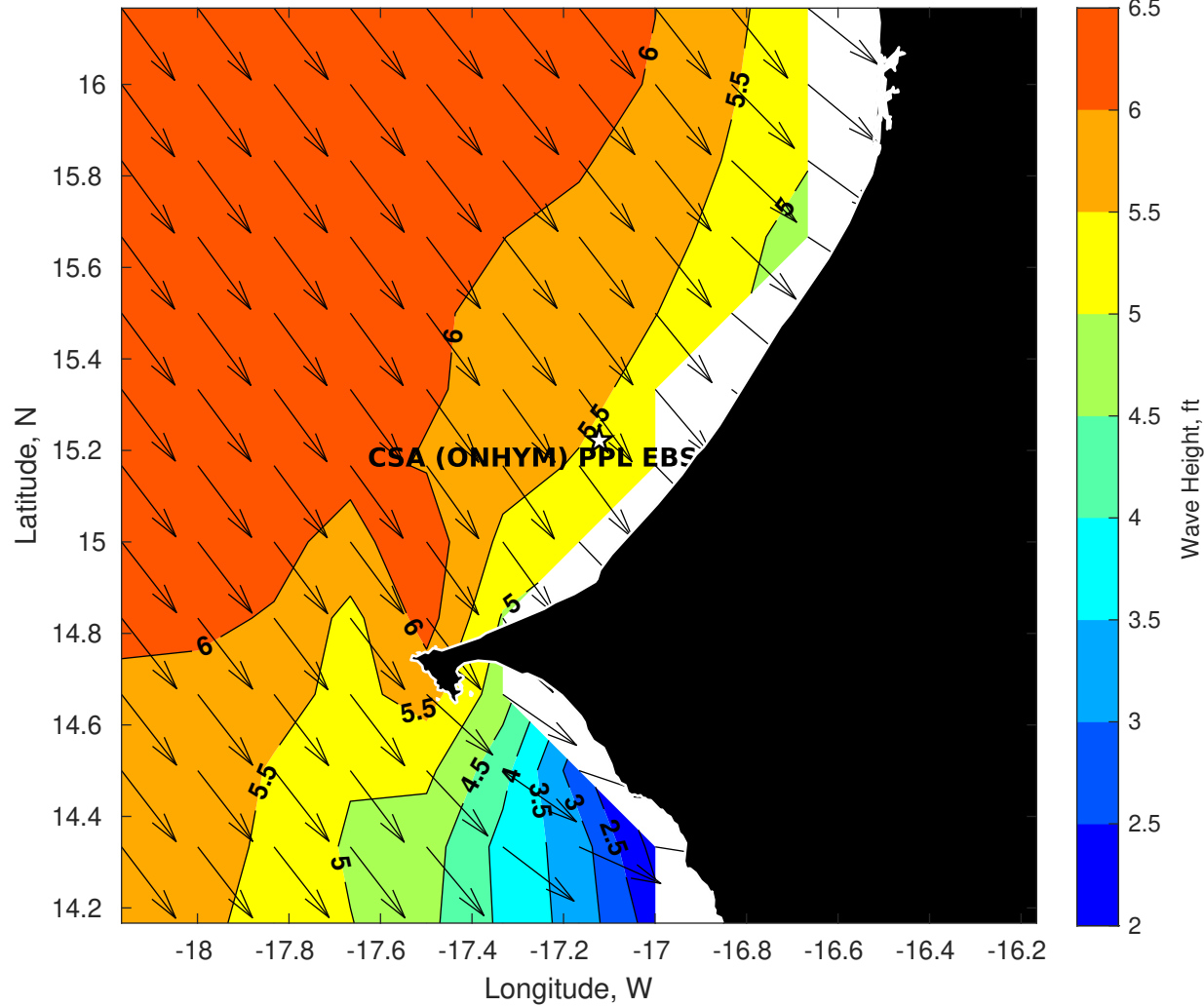
Wave Height (ft) for CSA (ONHYM) PPL EBS - Senegal at 27-Apr-2025 09:00:00
