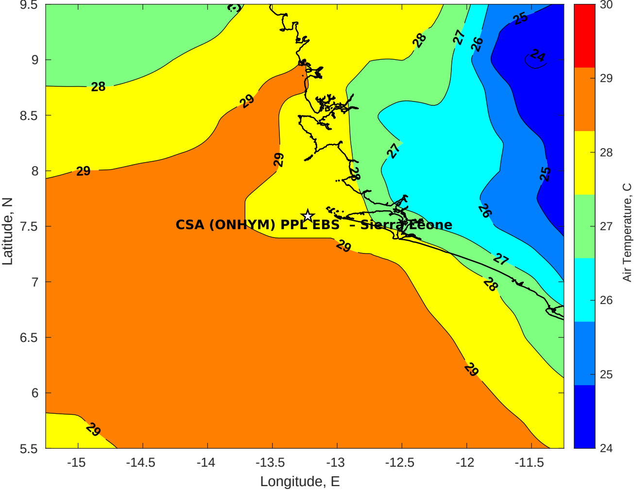
Air Temperature (C) for CSA (ONHYM) PPL EBS - Sierra Leone at 27-Apr-2025
