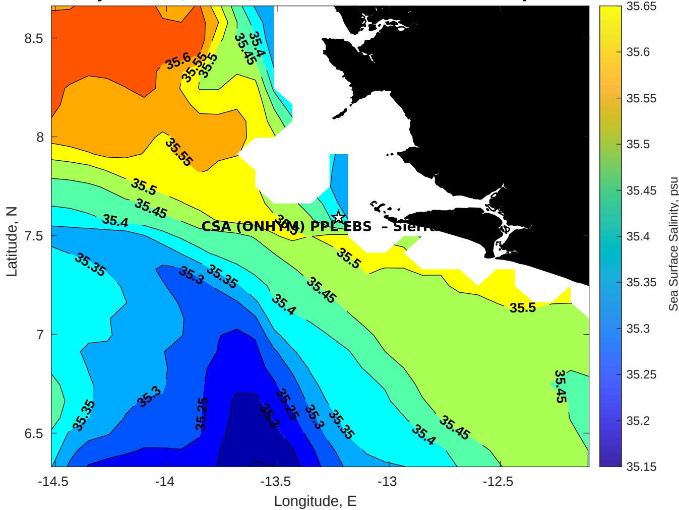
Surface Salinity for CSA (ONHYM) PPL EBS - Sierra Leone at 26-Apr-2025 00:00:00
