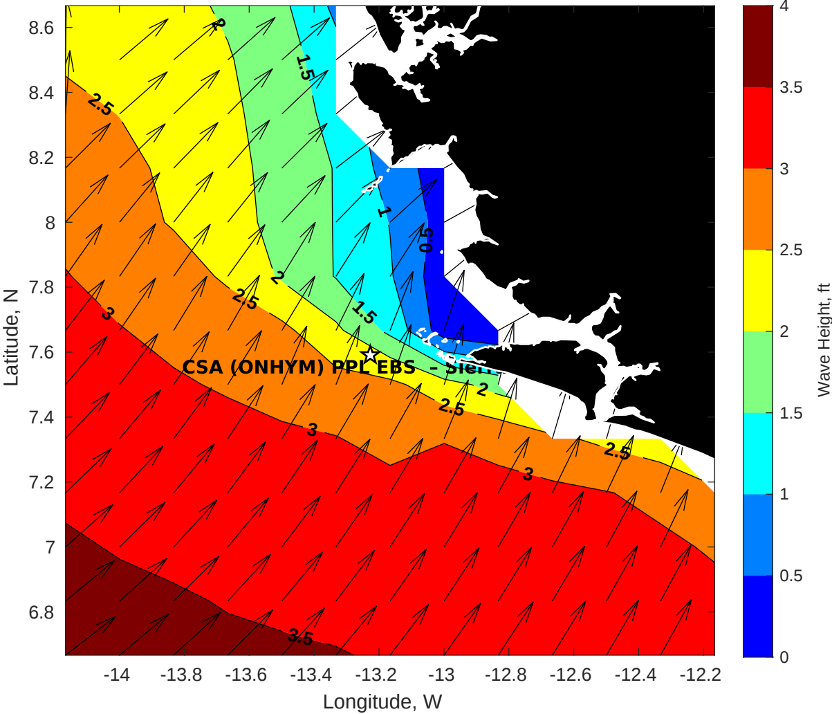
Wave Height (ft) for CSA (ONHYM) PPL EBS - Sierra Leone at 27-Apr-2025 09:00:00
