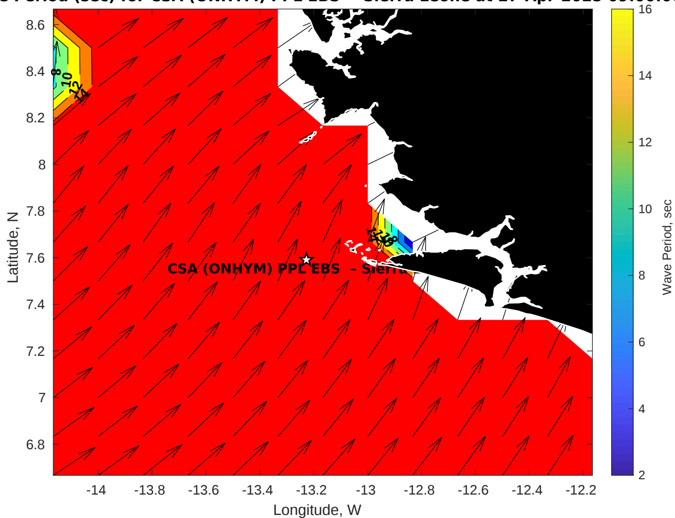
Wave Period (sec) for CSA (ONHYM) PPL EBS - Sierra Leone at 27-Apr-2025 09:00:00
