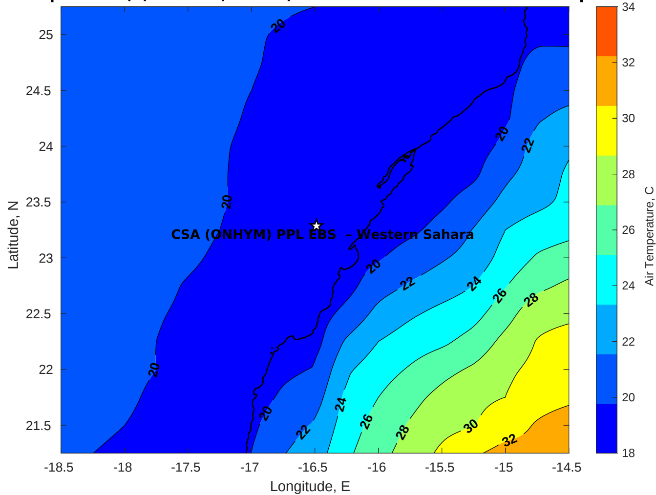
Air Temperature (C) for CSA (ONHYM) PPL EBS - Western Sahara at 27-Apr-2025
