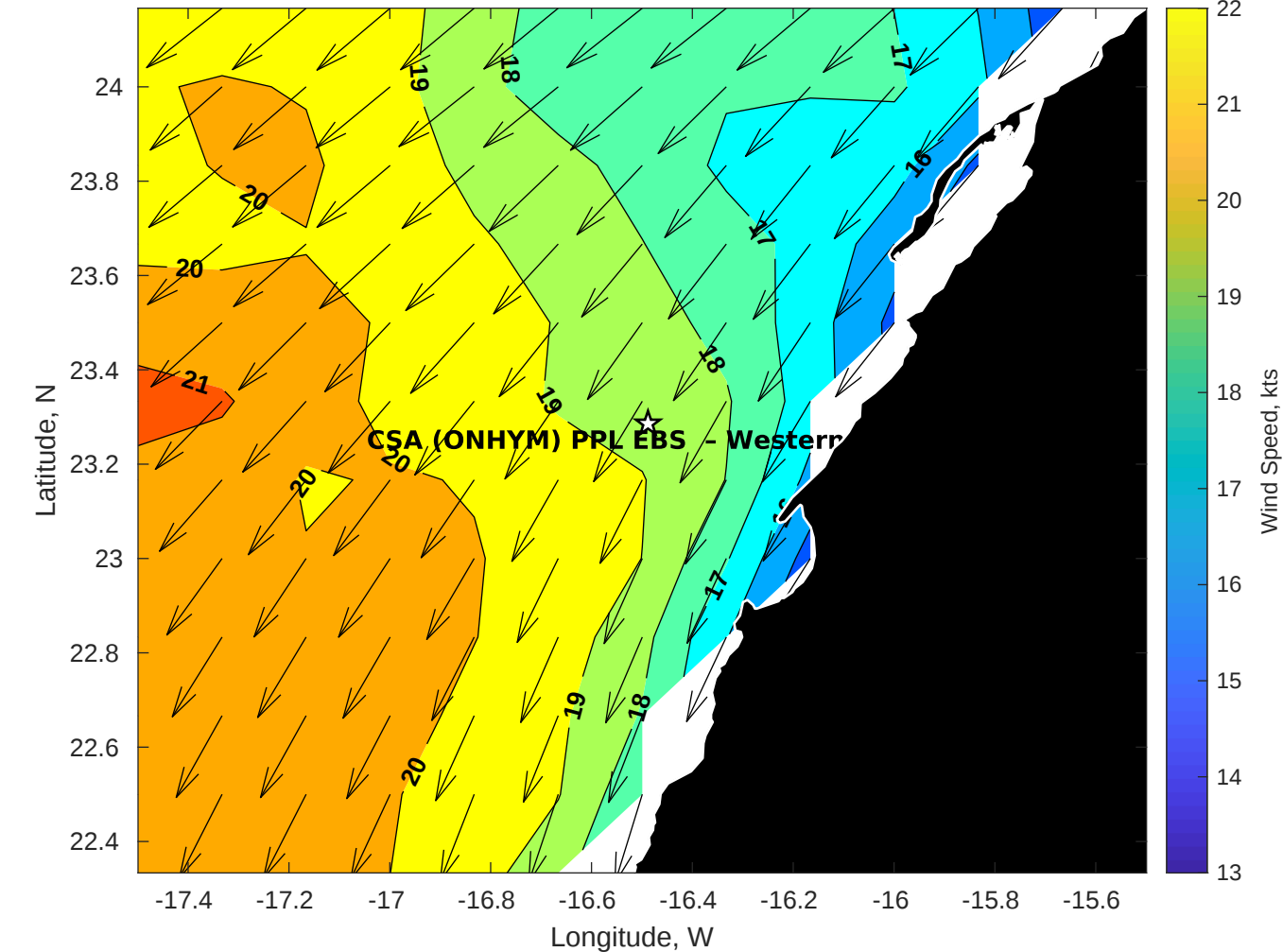
Winds (kts) for CSA (ONHYM) PPL EBS - Western Sahara at 27-Apr-2025 09:00:00
