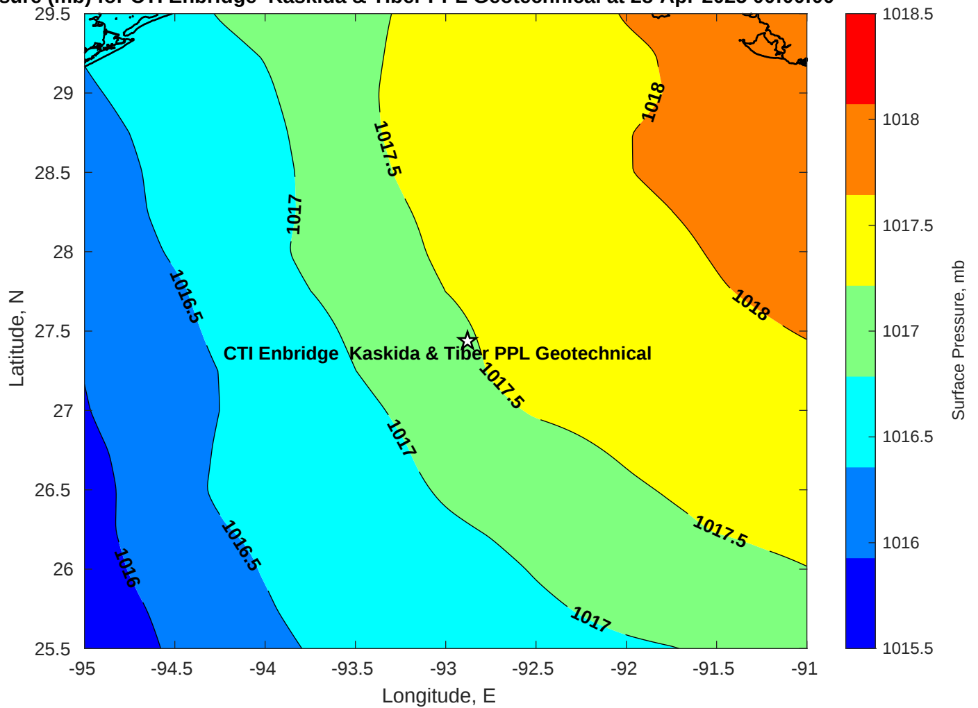
Surface Pressure (mb) for CTI Enbridge Kaskida & Tiber PPL Geotechnical at 28-Apr-2025 00:00:00
