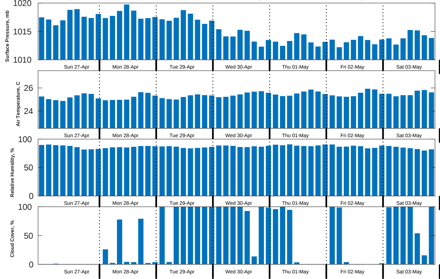
Met Forecast for CTI Enbridge Kaskida & Tiber PPL Geotechnical from 27-Apr-2025 00:00:00 to 04-May-2025 00:00:00
