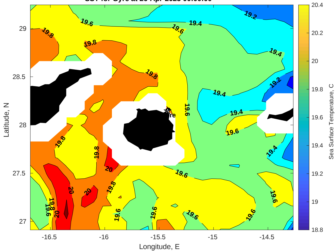
SST for Gyre at 26-Apr-2025 00:00:00
