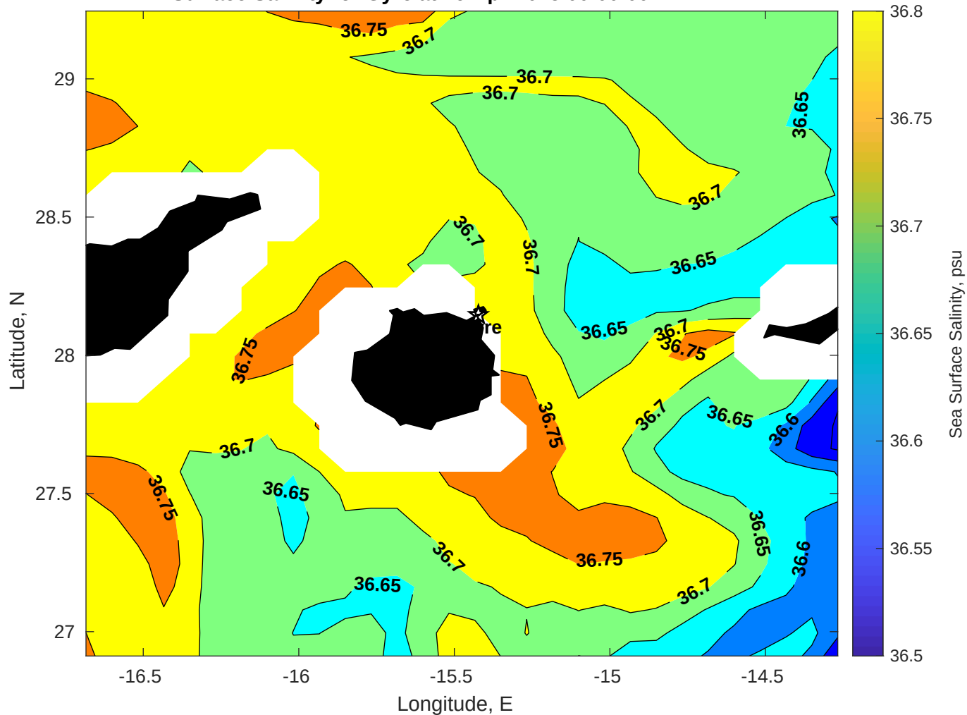
Surface Salinity for Gyre at 26-Apr-2025 00:00:00
