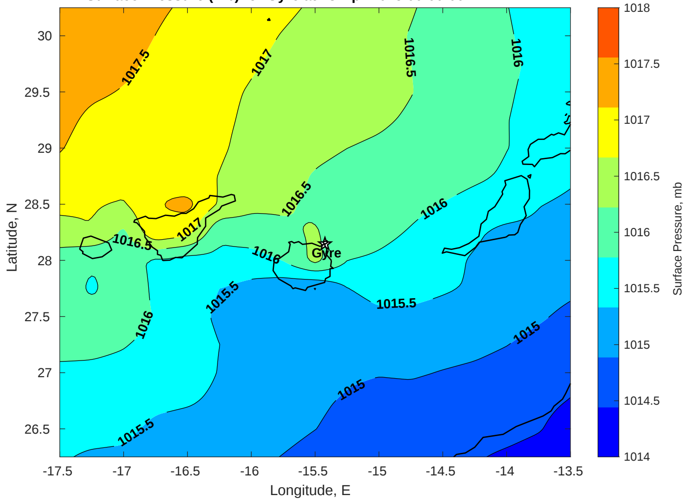
Surface Pressure (mb) for Gyre at 28-Apr-2025 00:00:00
