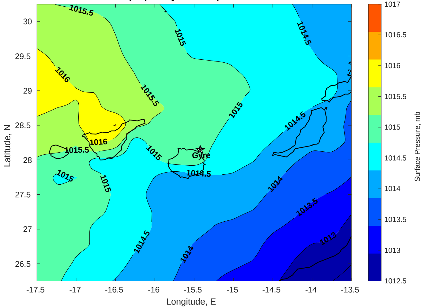
Surface Pressure (mb) for Gyre at 29-Apr-2025 00:00:00
