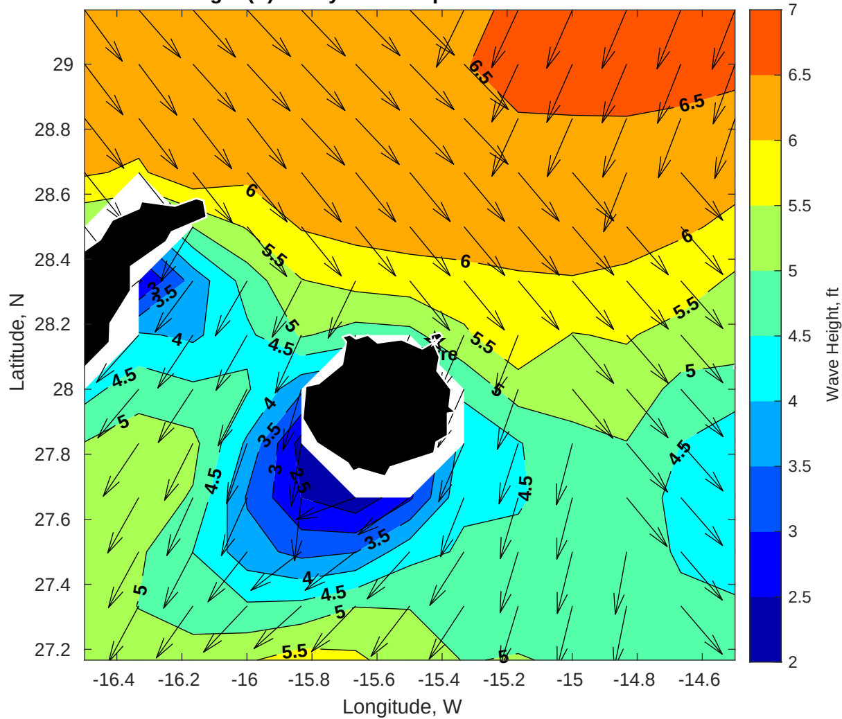
Wave Height (ft) for Gyre at 27-Apr-2025 09:00:00
