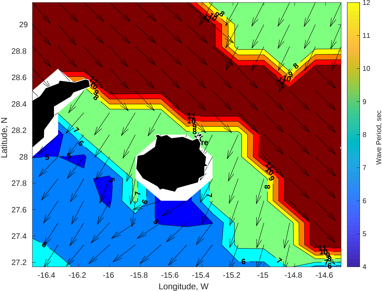
Wave Period (sec) for Gyre at 27-Apr-2025 09:00:00
