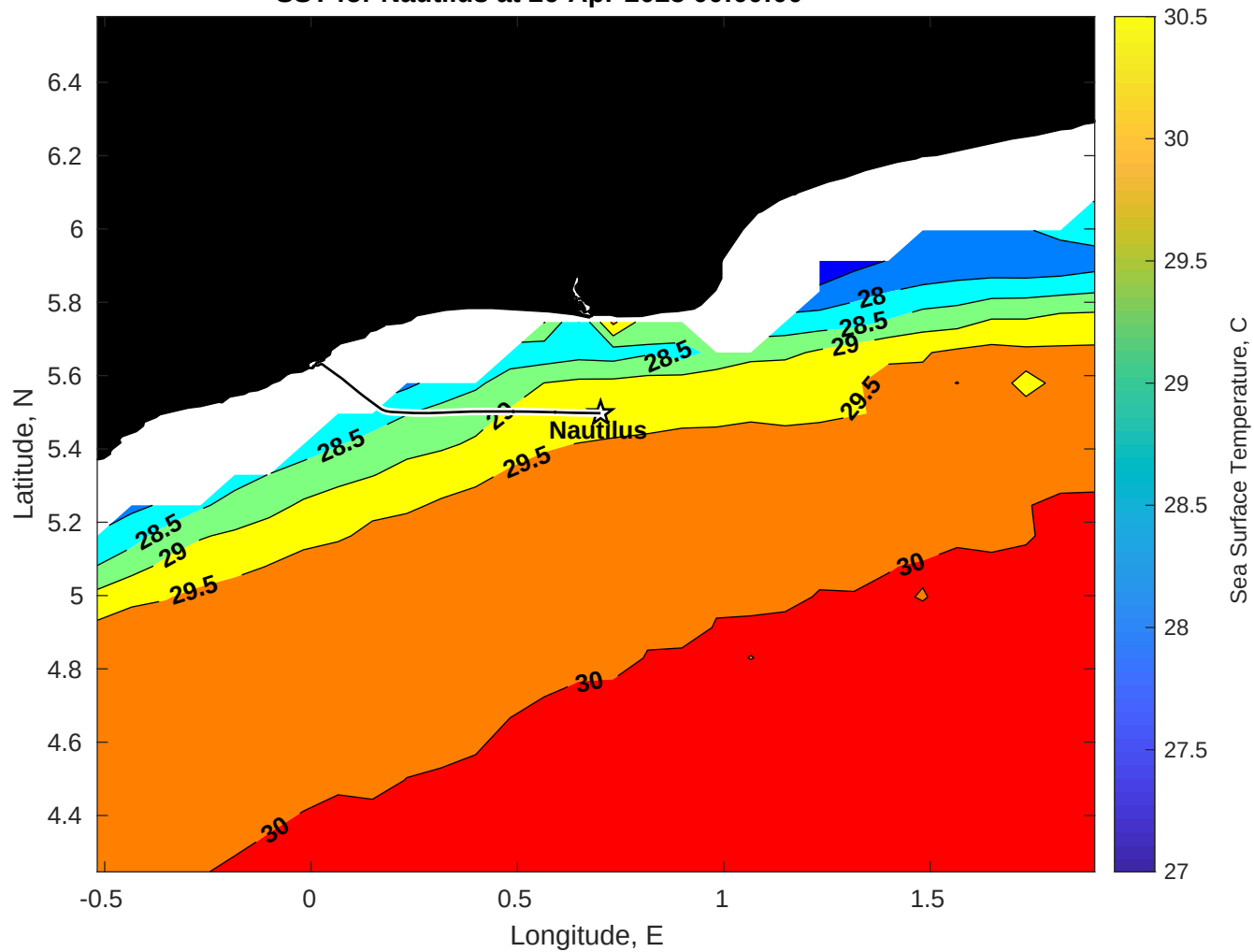
SST for Nautilus at 26-Apr-2025 00:00:00
