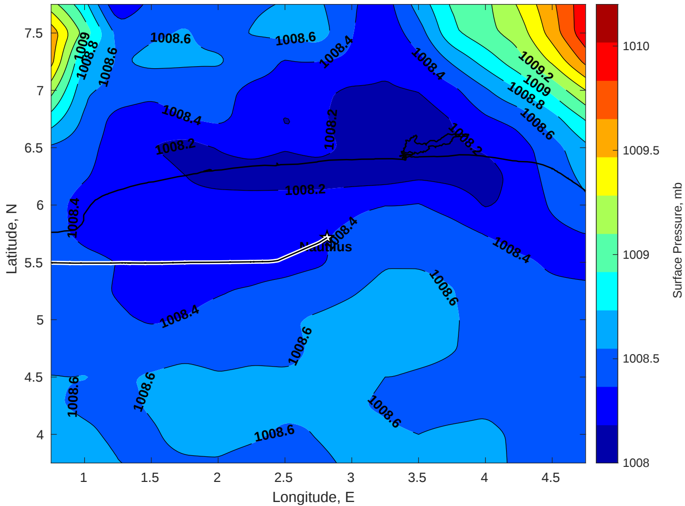
Surface Pressure (mb) for Nautilus at 29-Apr-2025 00:00:00
