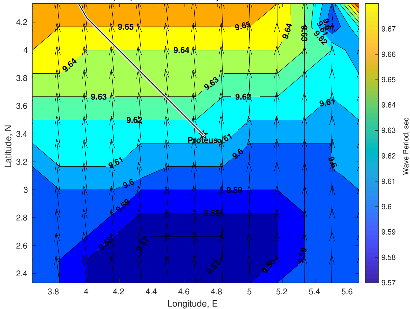
Wave Period (sec) for Proteus at 27-Apr-2025 09:00:00
