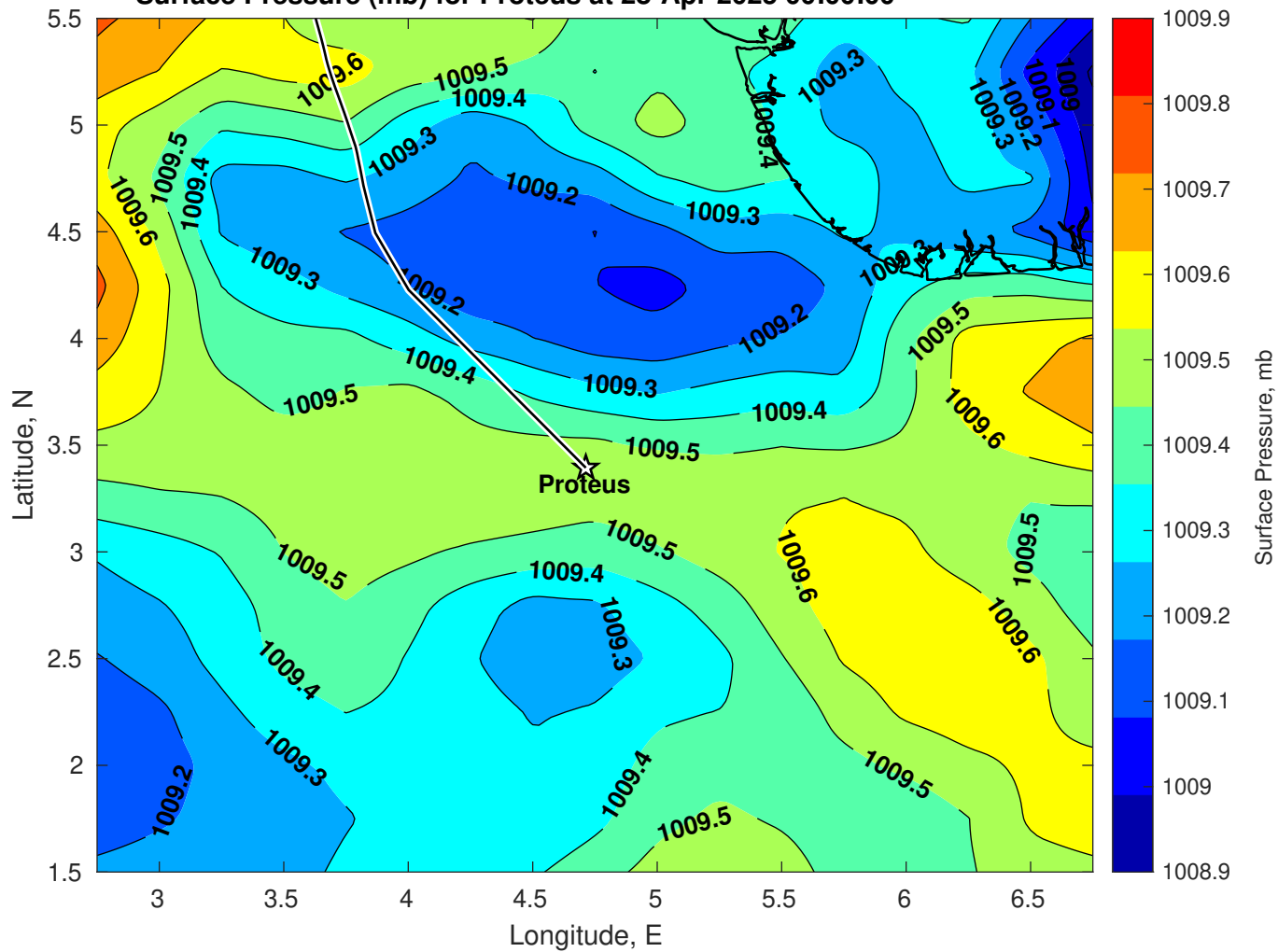
Surface Pressure (mb) for Proteus at 28-Apr-2025 00:00:00
