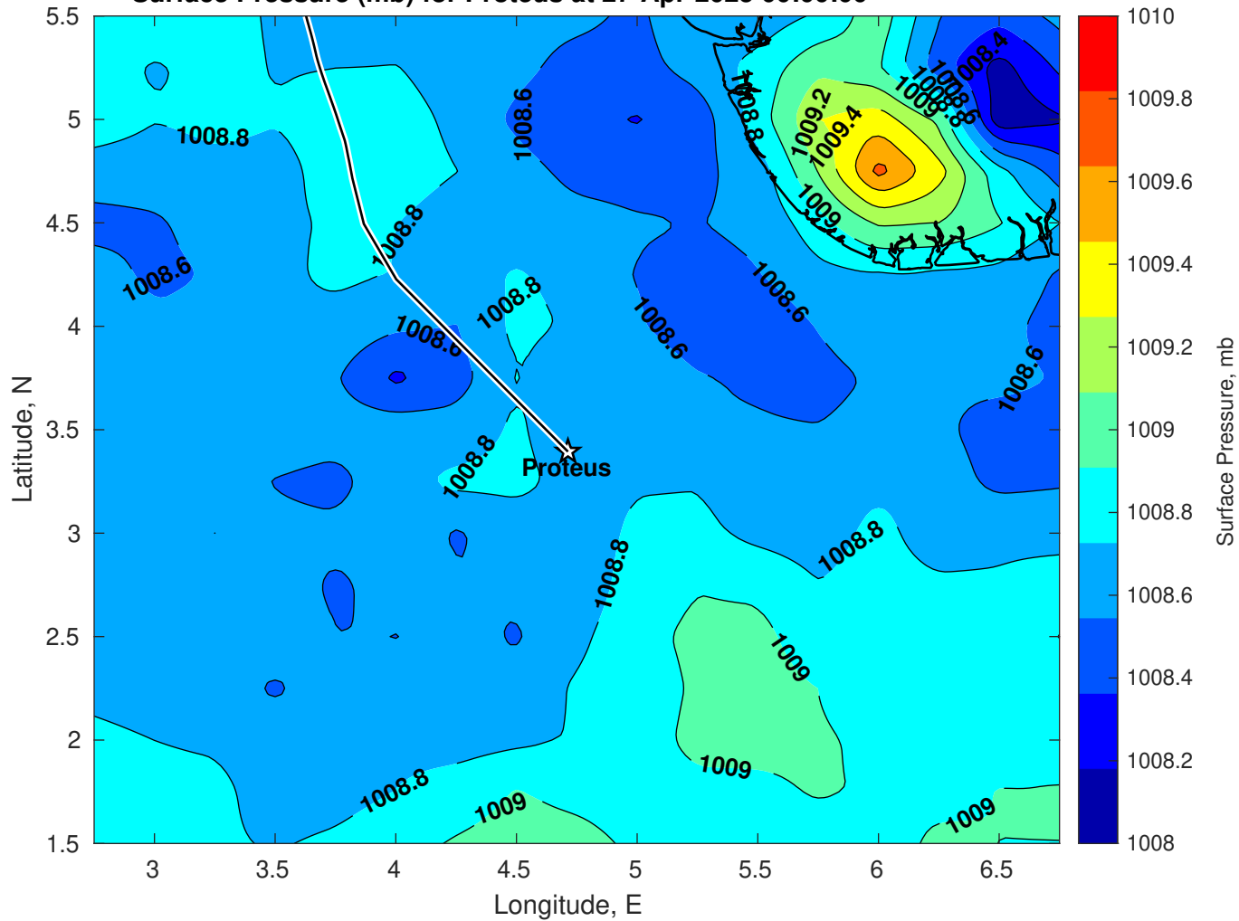
Surface Pressure (mb) for Proteus at 27-Apr-2025 00:00:00
