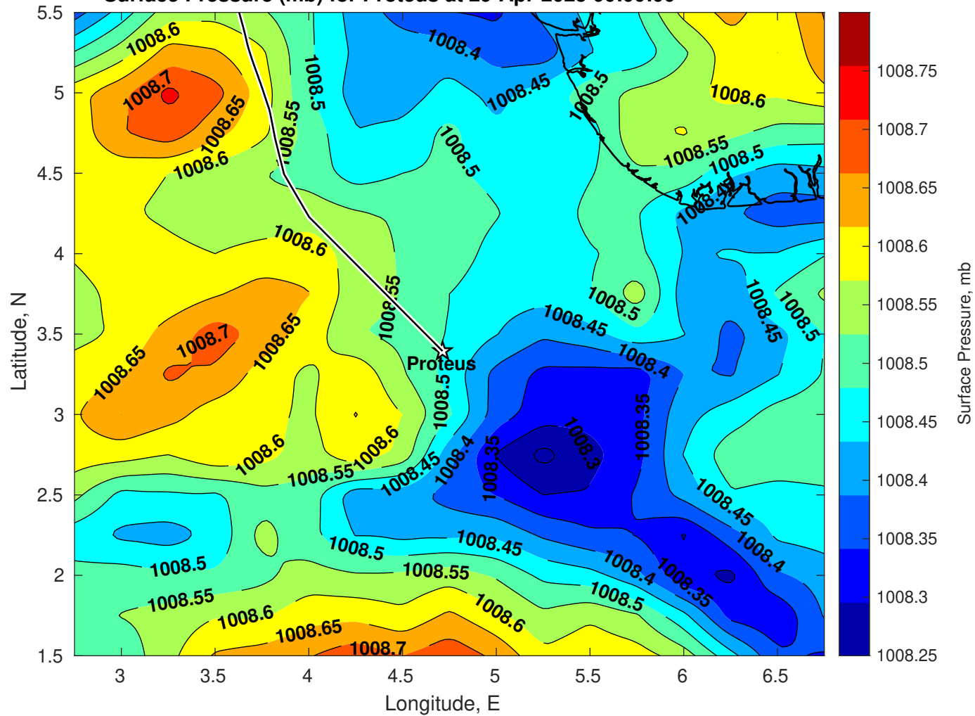
Surface Pressure (mb) for Proteus at 29-Apr-2025 00:00:00
