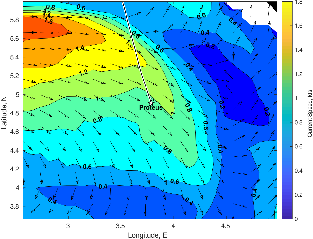
Surface Currents for Proteus at 26-Apr-2025 00:00:00
