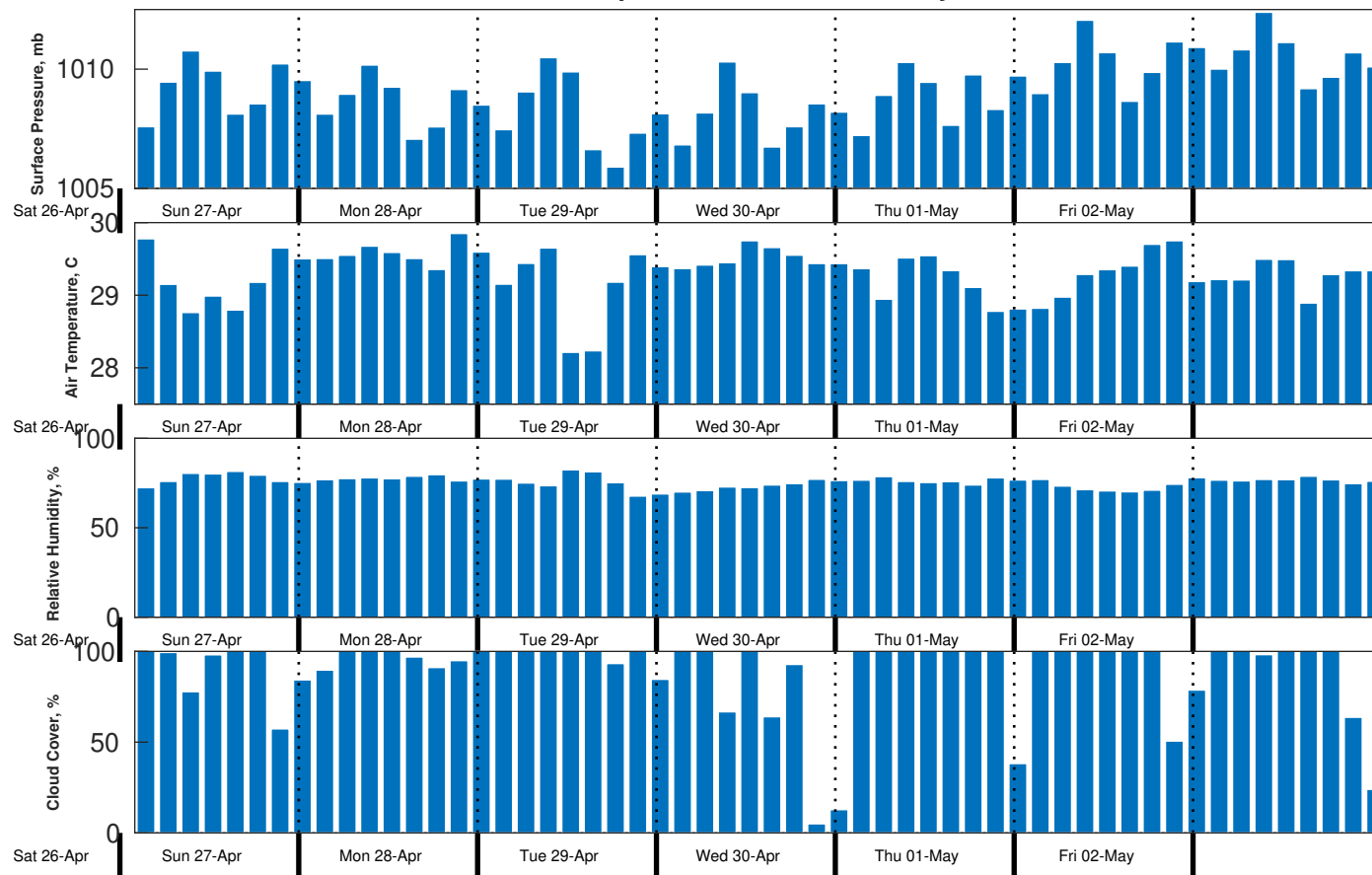
Met Forecast for Proteus from 27-Apr-2025 00:00:00 to 04-May-2025 00:00:00
