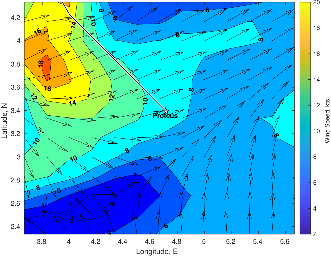
Winds (kts) for Proteus at 27-Apr-2025 09:00:00
