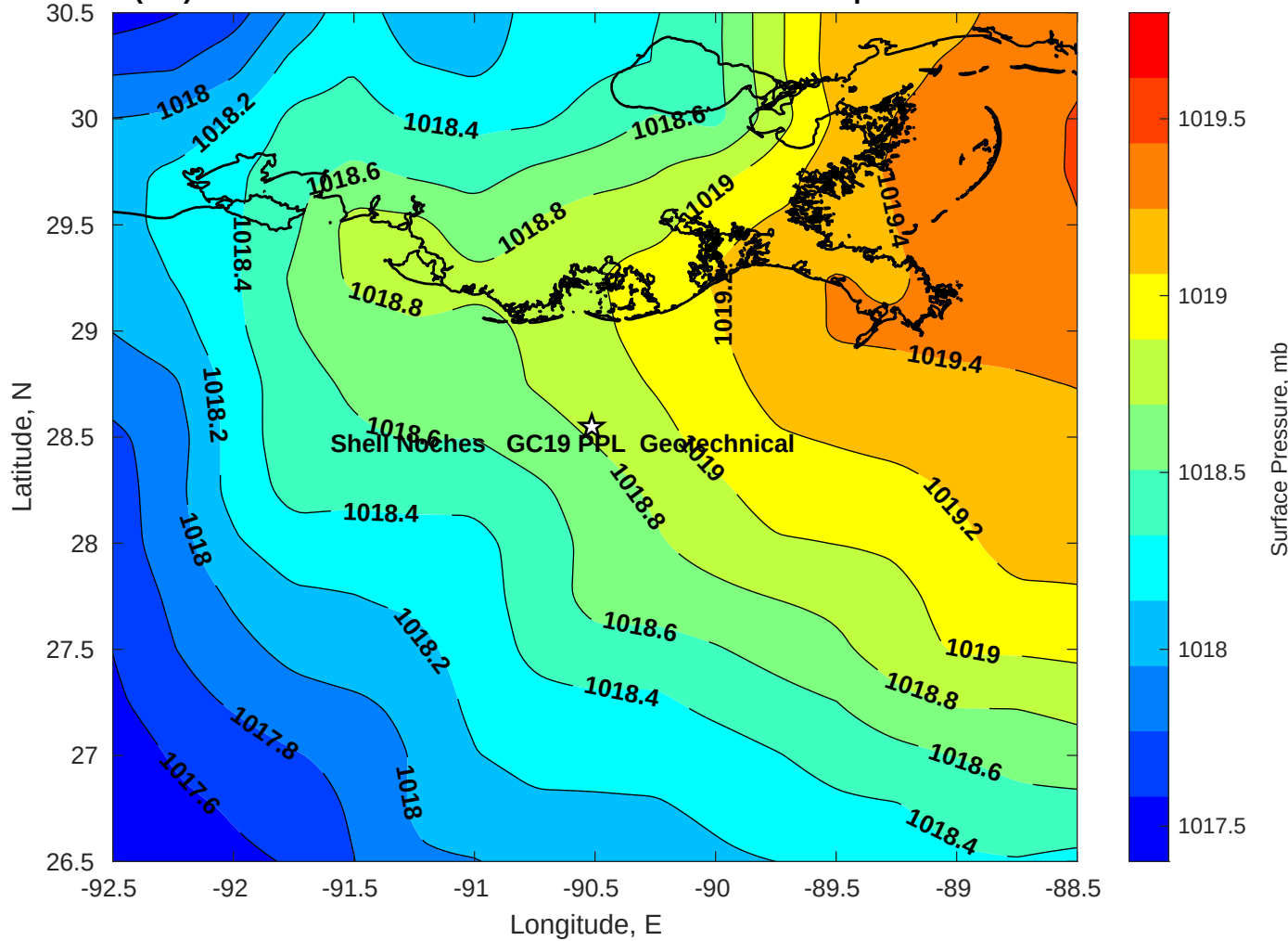
Surface Pressure (mb) for Shell Noches GC19 PPL Geotechnical at 29-Apr-2025 00:00:00
