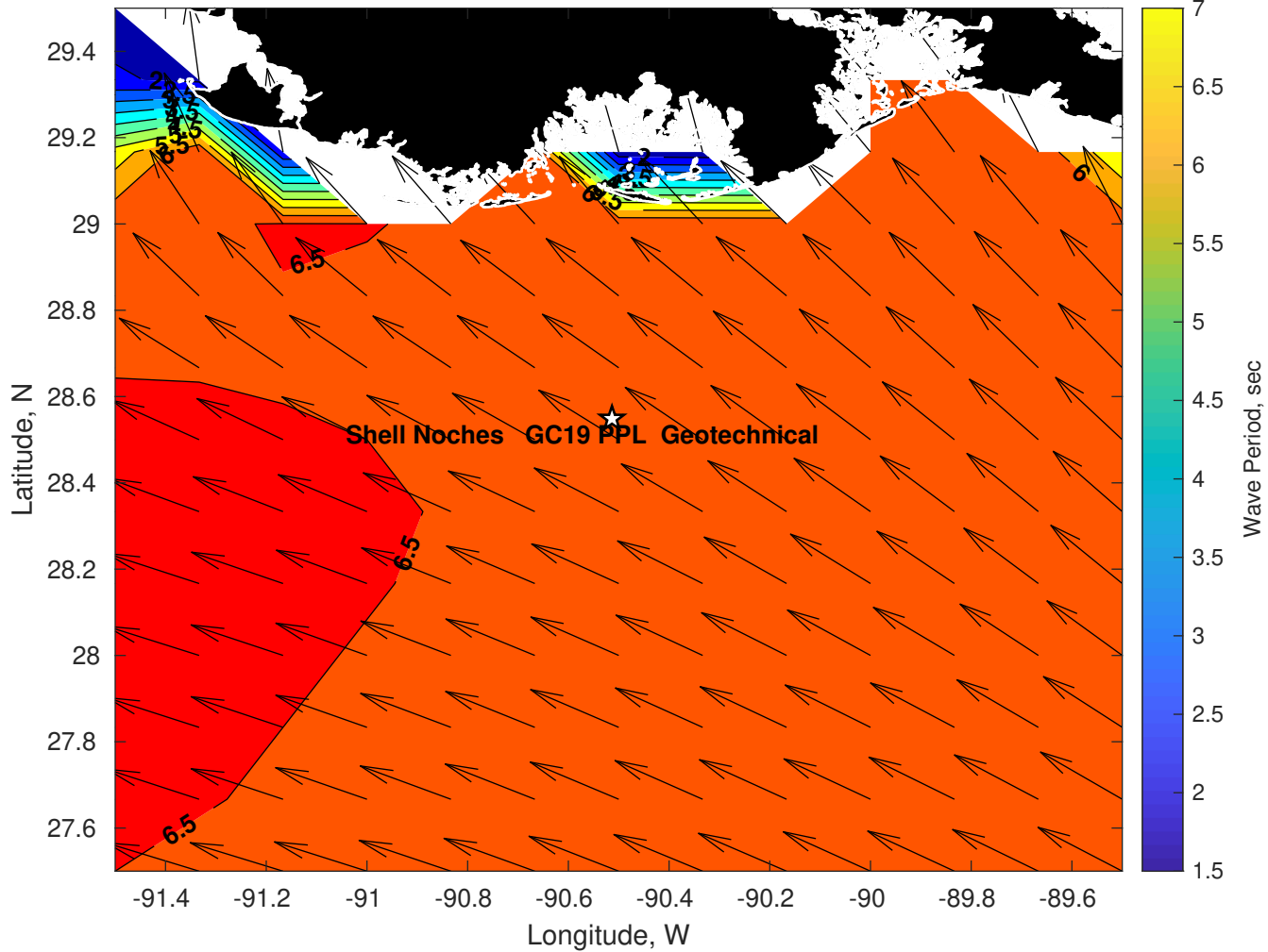
Wave Period (sec) for Shell Noches GC19 PPL Geotechnical at 27-Apr-2025 09:00:00
