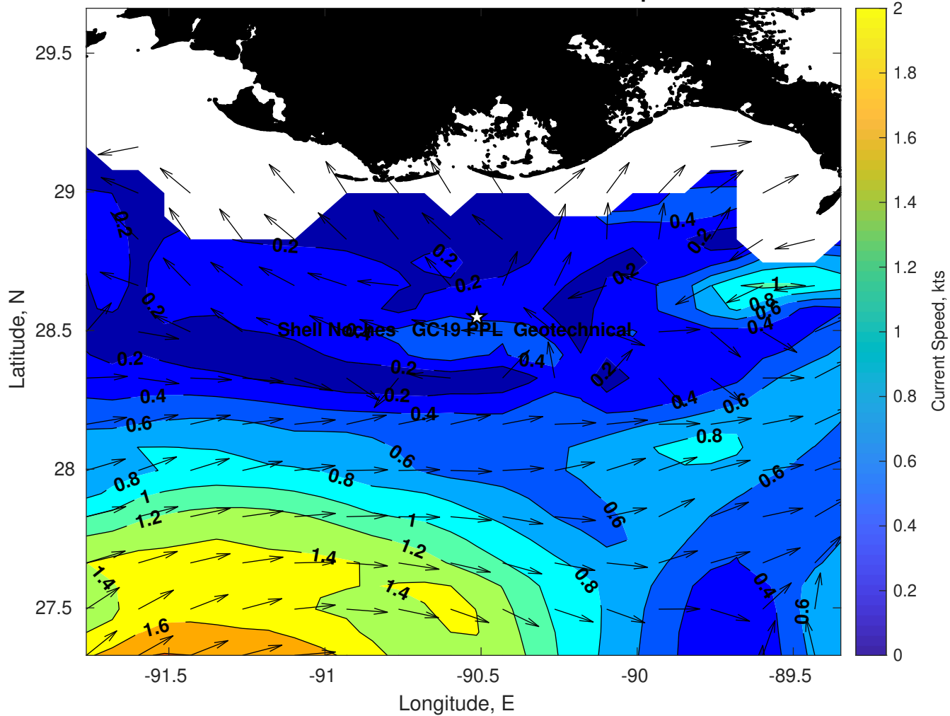
Surface Currents for Shell Noches GC19 PPL Geotechnical at 26-Apr-2025 00:00:00
