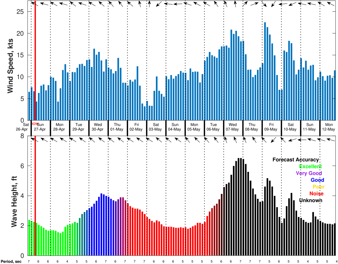
Wind & Wave Forecast for Shell Noches GC19 PPL Geotechnical from 26-Apr-2025 20:00:00 to 12-May-2025 20:00:00
