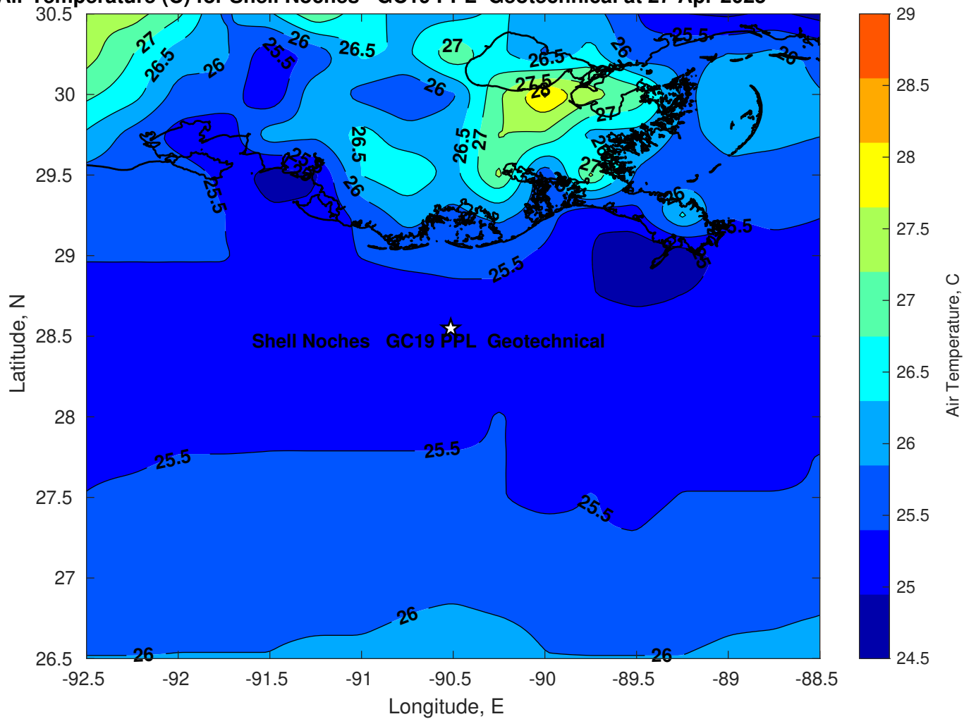
Air Temperature (C) for Shell Noches GC19 PPL Geotechnical at 27-Apr-2025
