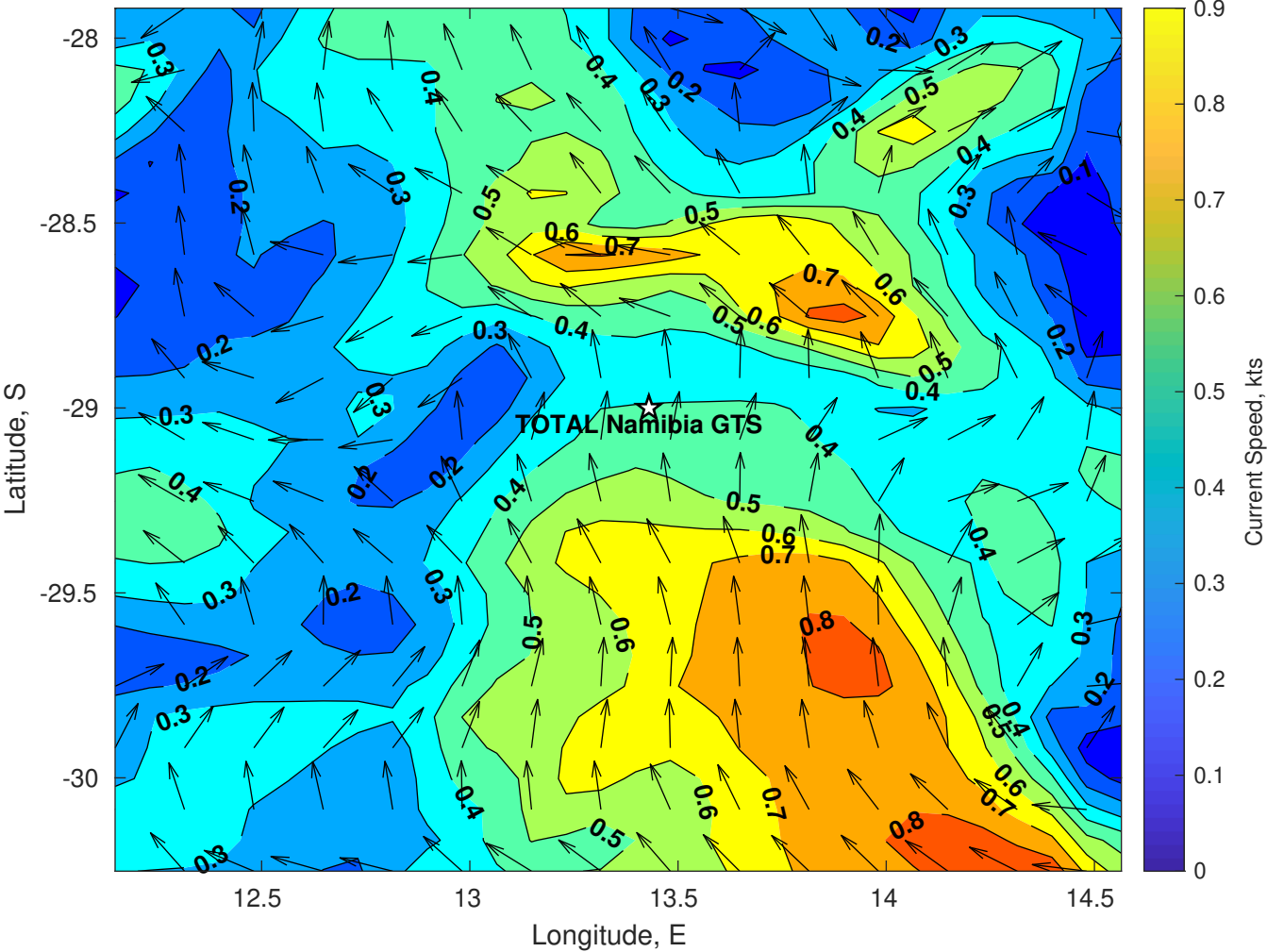
Surface Currents for TOTAL Namibia GTS at 26-Apr-2025 00:00:00
