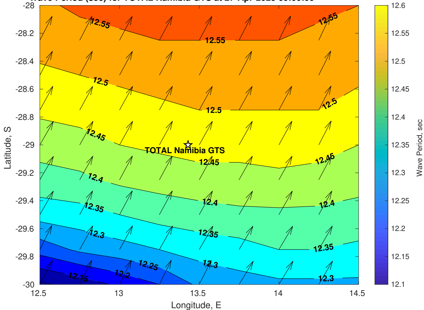
Wave Period (sec) for TOTAL Namibia GTS at 27-Apr-2025 09:00:00
