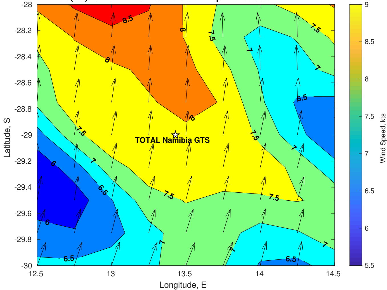
Winds (kts) for TOTAL Namibia GTS at 27-Apr-2025 09:00:00
