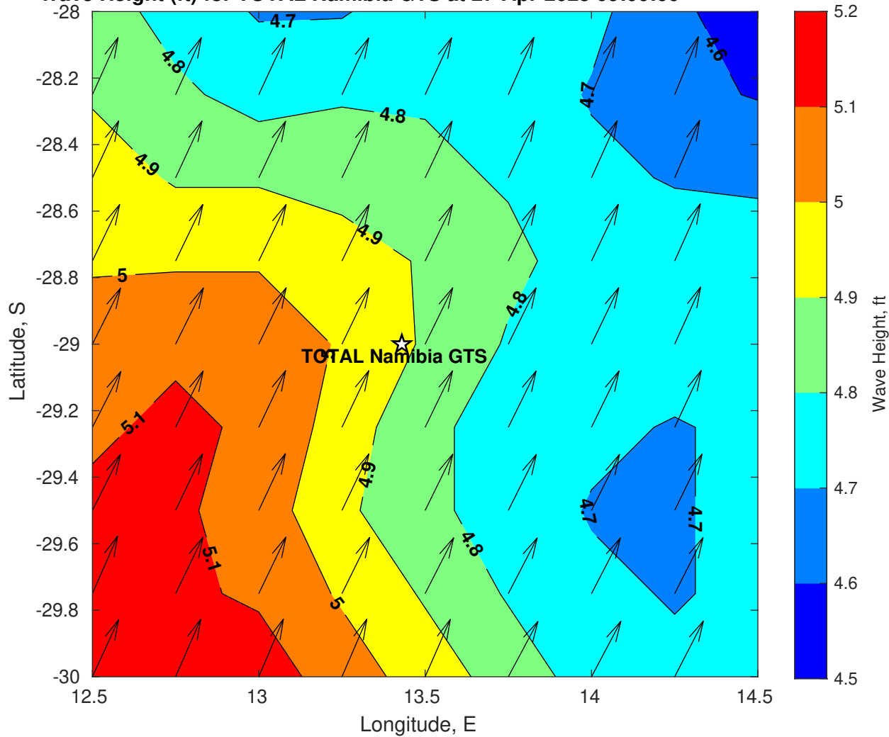
Wave Height (ft) for TOTAL Namibia GTS at 27-Apr-2025 09:00:00
