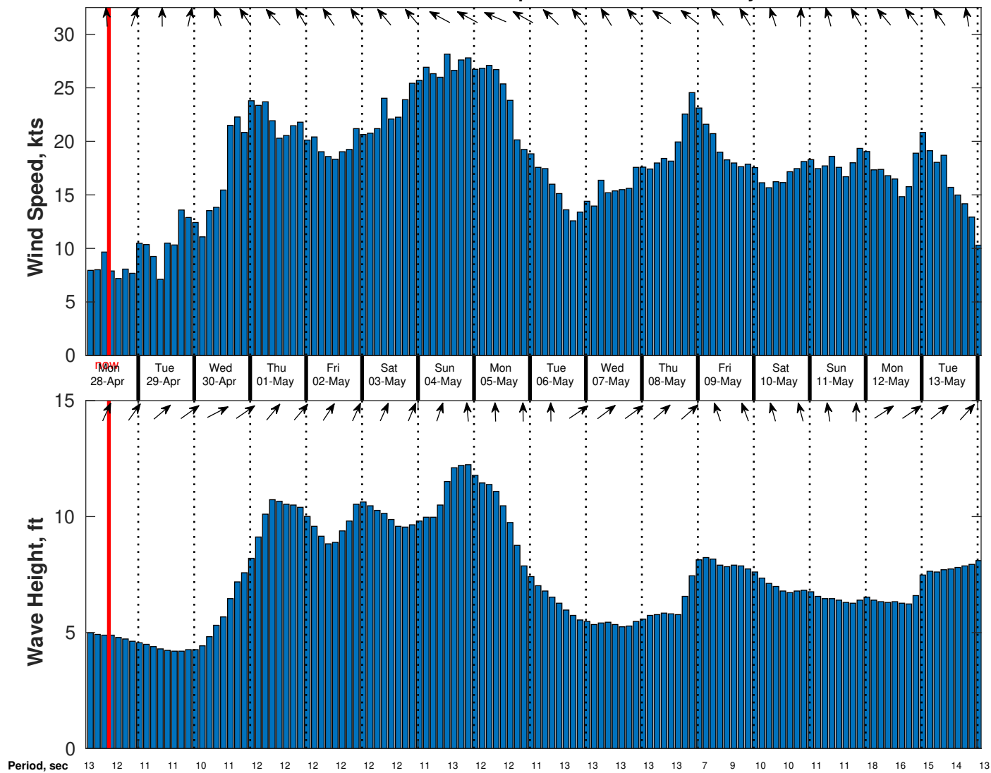
Wind & Wave Forecast for TOTAL Namibia GTS from 27-Apr-2025 02:00:00 to 13-May-2025 02:00:00
