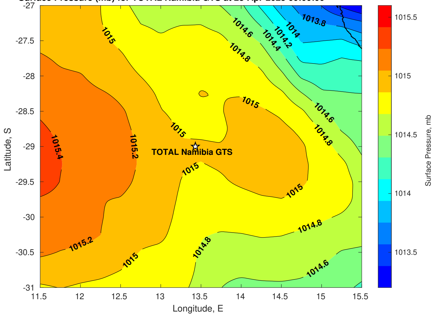
Surface Pressure (mb) for TOTAL Namibia GTS at 28-Apr-2025 00:00:00
