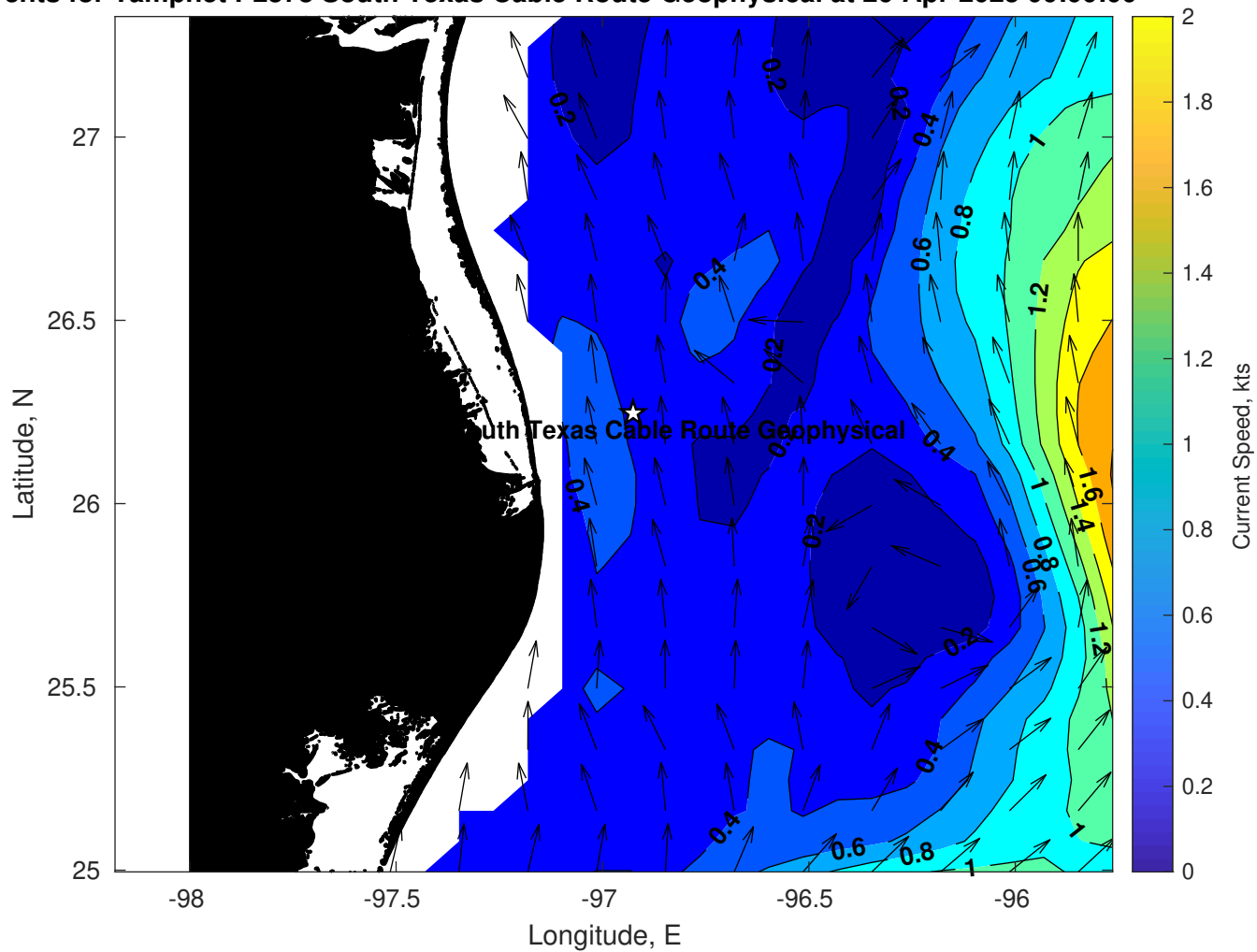
Surface Currents for Tampnet P2378 South Texas Cable Route Geophysical at 26-Apr-2025 00:00:00
