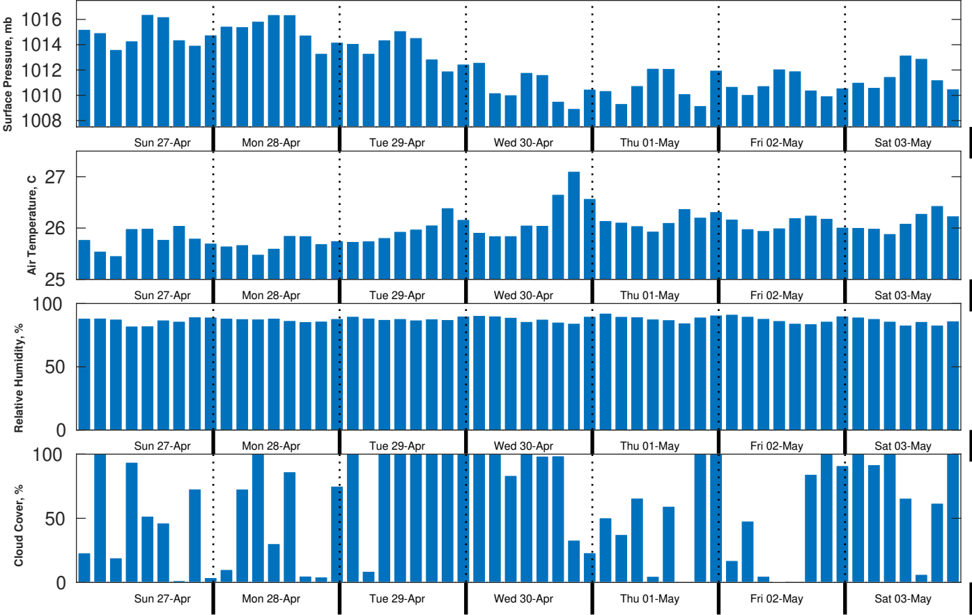
Met Forecast for Tampnet P2378 South Texas Cable Route Geophysical from 27-Apr-2025 00:00:00 to 04-May-2025 00:00:00
