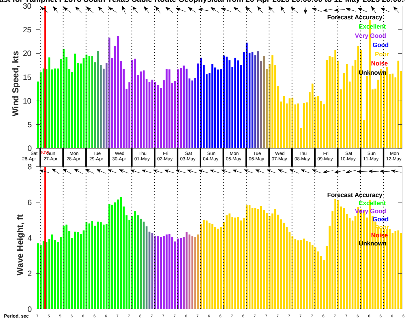
Wind & Wave Forecast for Tampnet P2378 South Texas Cable Route Geophysical from 26-Apr-2025 20:00:00 to 12-May-2025 20:00:00
