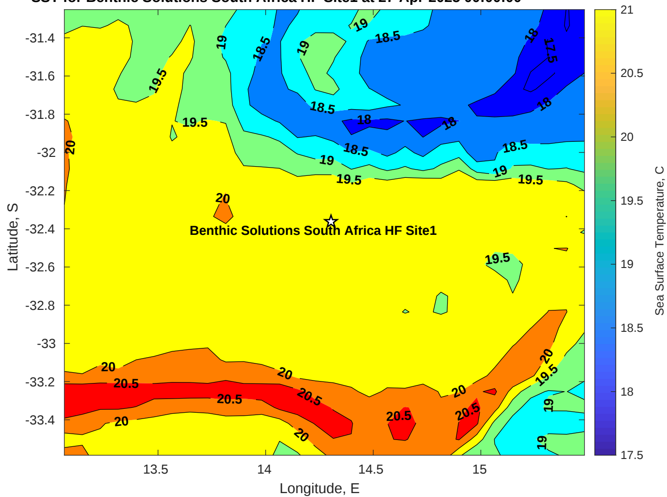
SST for Benthic Solutions South Africa HF Site1 at 27-Apr-2025 00:00:00
