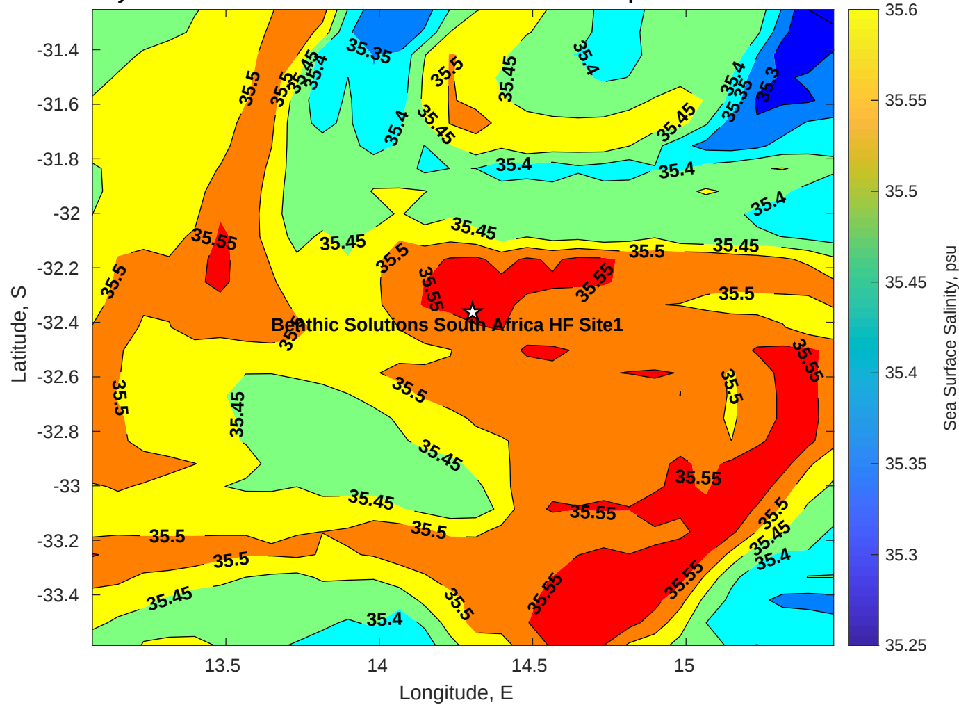
Surface Salinity for Benthic Solutions South Africa HF Site1 at 27-Apr-2025 00:00:00
