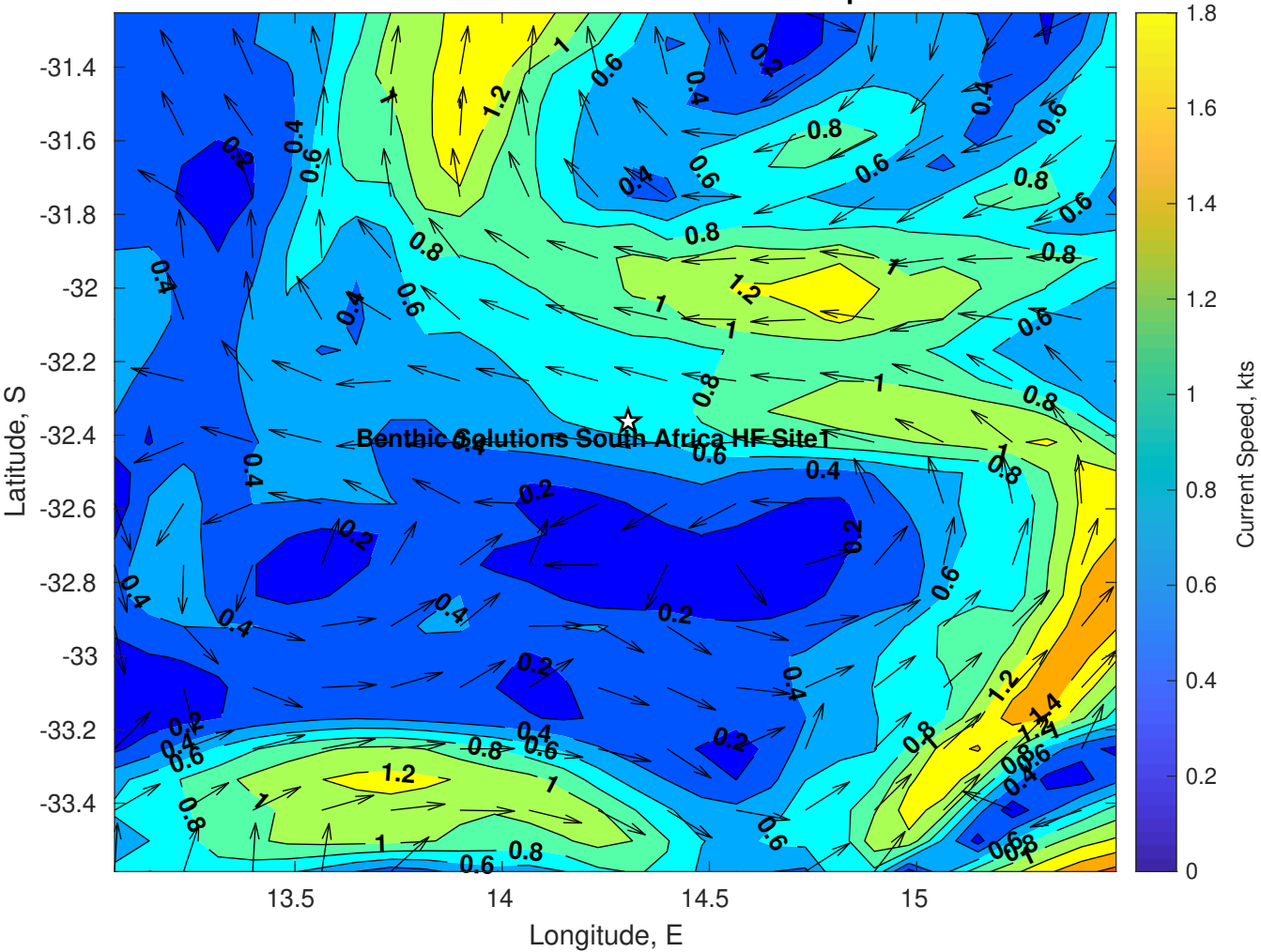
Surface Currents for Benthic Solutions South Africa HF Site1 at 27-Apr-2025 00:00:00
