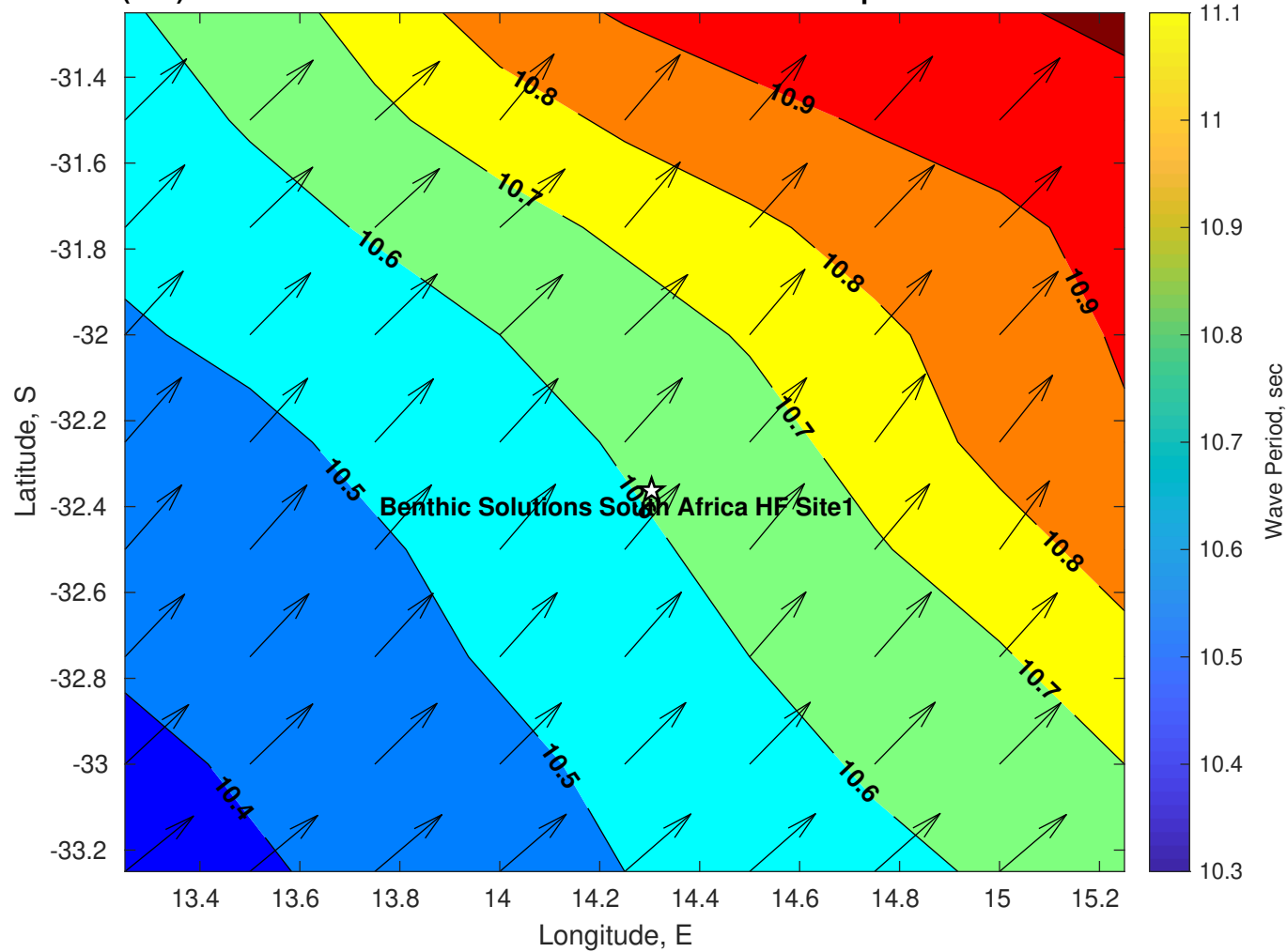
Wave Period (sec) for Benthic Solutions South Africa HF Site1 at 28-Apr-2025 09:00:00
