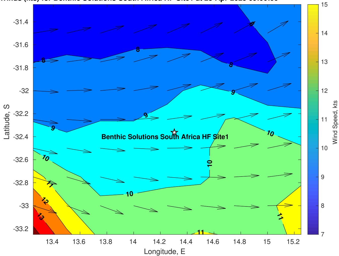
Winds (kts) for Benthic Solutions South Africa HF Site1 at 28-Apr-2025 09:00:00
