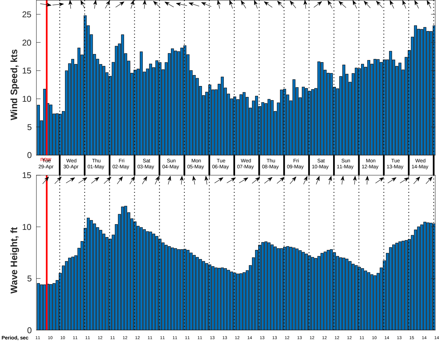
Wind & Wave Forecast for Benthic Solutions South Africa HF Site1 from 28-Apr-2025 02:00:00 to 14-May-2025 02:00:00
