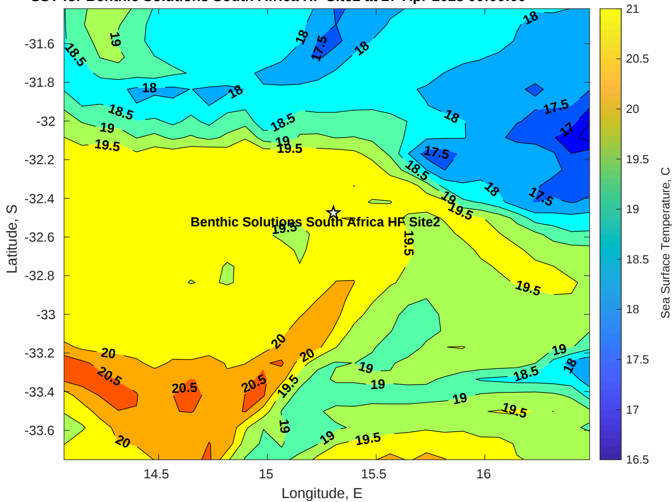
SST for Benthic Solutions South Africa HF Site2 at 27-Apr-2025 00:00:00
