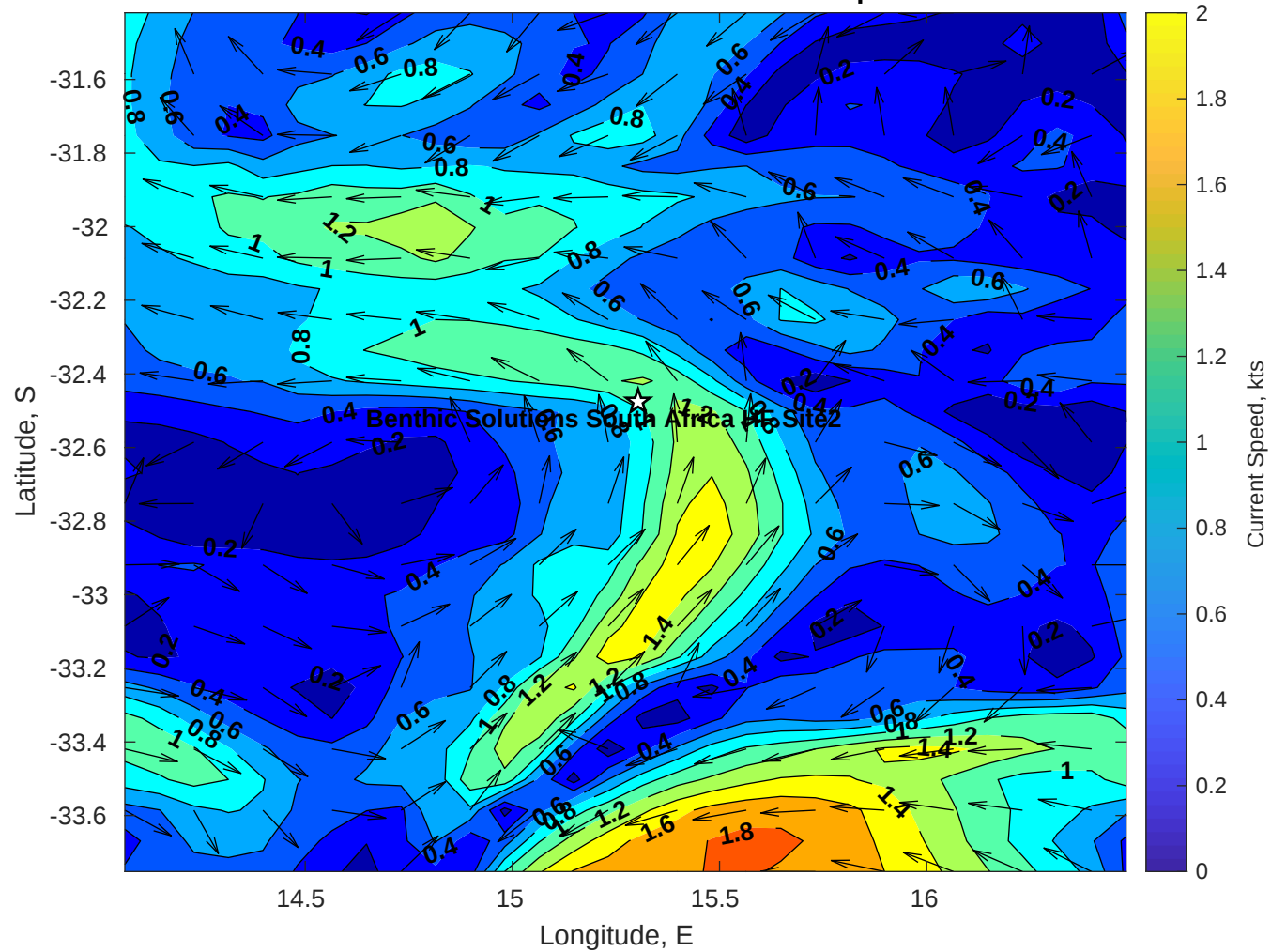
Surface Currents for Benthic Solutions South Africa HF Site2 at 27-Apr-2025 00:00:00
