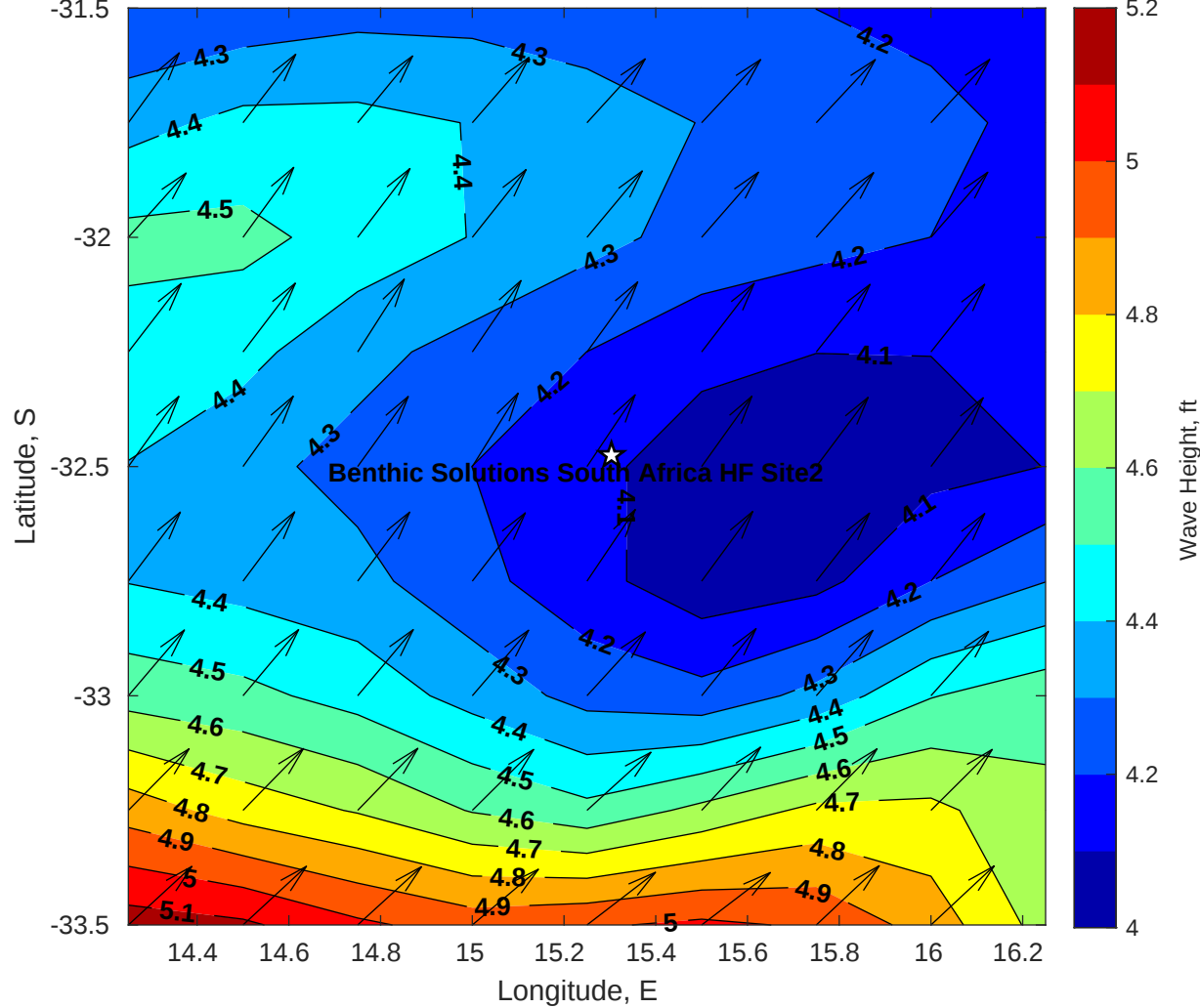
Wave Height (ft) for Benthic Solutions South Africa HF Site2 at 28-Apr-2025 09:00:00
