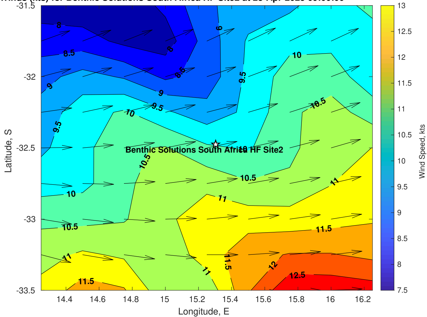
Winds (kts) for Benthic Solutions South Africa HF Site2 at 28-Apr-2025 09:00:00
