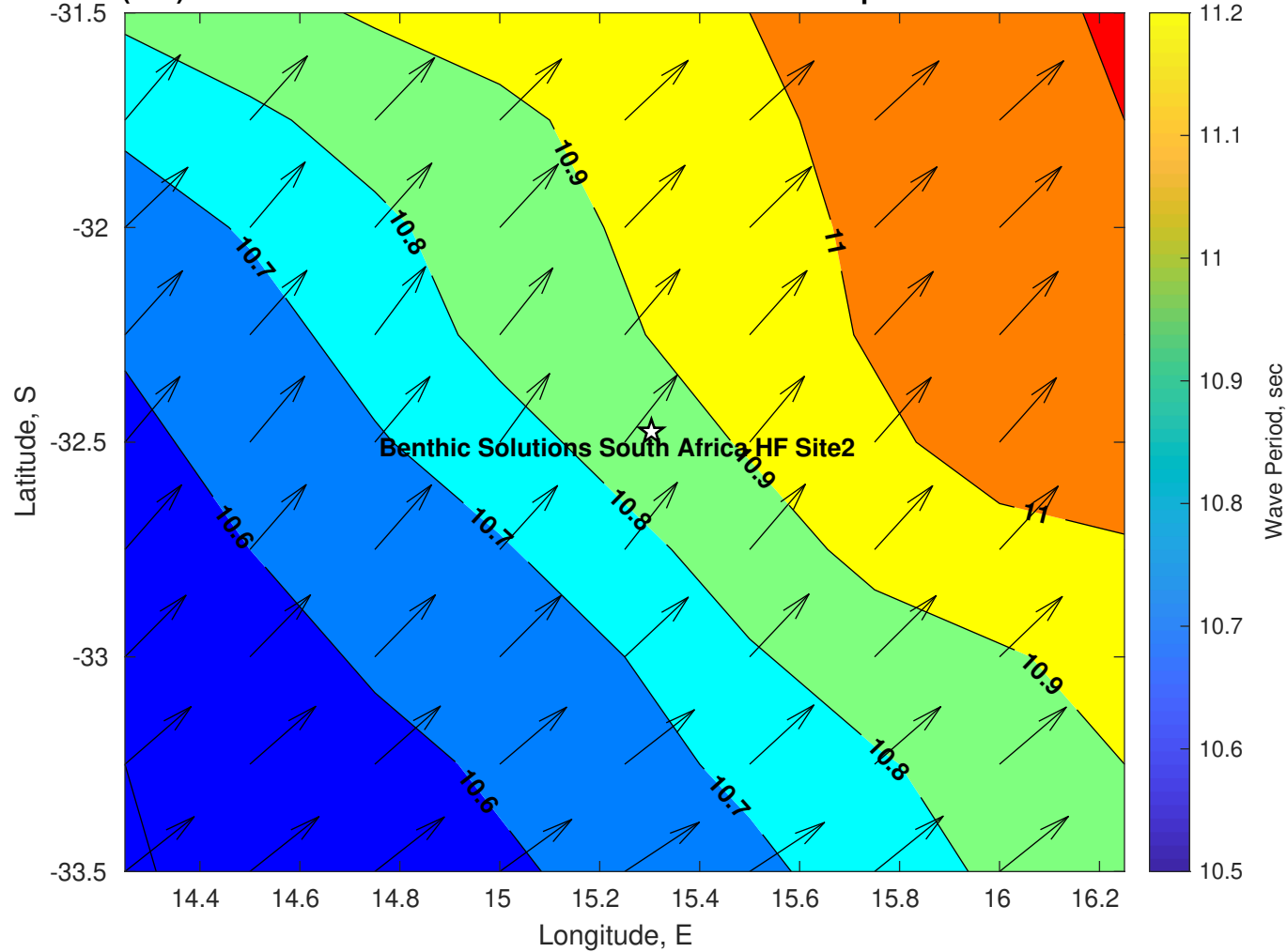
Wave Period (sec) for Benthic Solutions South Africa HF Site2 at 28-Apr-2025 09:00:00
