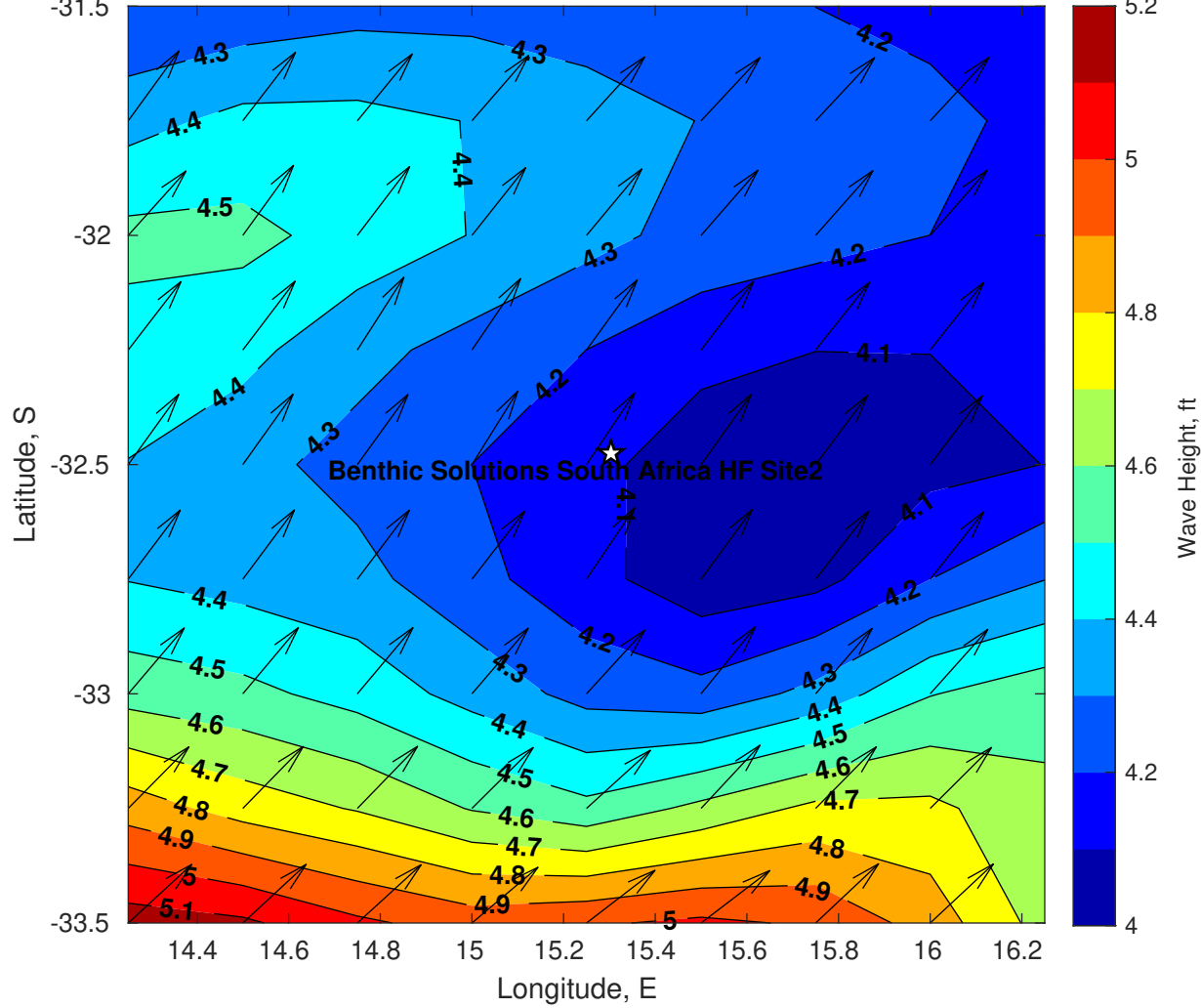
Wave Height (ft) for Benthic Solutions South Africa HF Site2 at 28-Apr-2025 09:00:00
